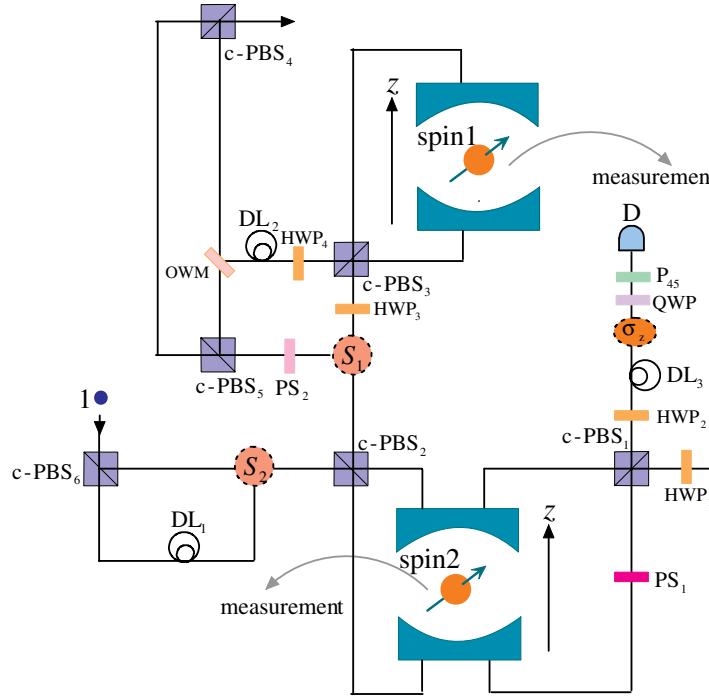
Figure 3. Schematic of photonic W-state fusion. All the optical elements are the same as Fig. 2.
