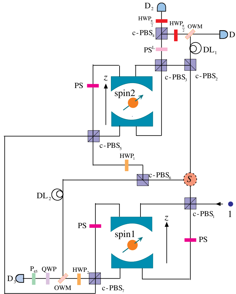
Figure 2. Schematic of electronic W -state. Spin 1 and spin 2 denote two QD spins coupled with two optical microcavities, respectively. c\text{-PBS}_i ( i = 1, 2, 3, \dots ): polarizing beam splitter in the circular basis. \text{HWP}_i is half-wave plate, and \text{HWP}_{\frac{\pi}{2}} implements the transformation |R\rangle \leftrightarrow |L\rangle . QWP: quarter-wave plate. S: optical switch. PS: \pi -phase shifter. The \text{PS}^L introduces a \pi phase for |L\rangle and does not affect |R\rangle . OWM: one-way mirror transmits photons from one side, and reflects photons from the other side without remodulating. P_{45} is a 45^\circ polarizer projecting the polarization to (|H\rangle + |V\rangle)/\sqrt{2} . \text{DL}_i : the time-delay device for matching pathes length of the different components of the same photon. D_i : conventional photon detectors.
