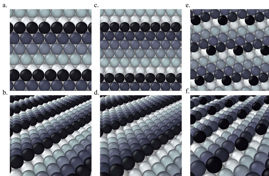
Fig. 1 Ball models of various clean surfaces considered. (a) Pt(553) top view, (b) Pt(553) side view, (c) Pt(557) top view, (d) Pt(557) side view, (e) Pt(643) top view, and (f) Pt(643) side view. Colors represent the z-position of the atoms. Black balls represent the step edge and others represent the terrace.
