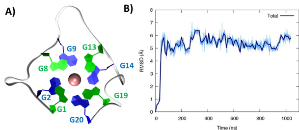
Fig. 1 A representative snapshot of the parallel G4 formed by the RG-2 sequence as obtained by MD simulations. Guanine residues composing the two superposing tetrads are evidenced by different colours (A). The corresponding time series of the RMSD for the RNA strand (B). Analogous results obtained for the second replica are reported in Fig. S3A.†
