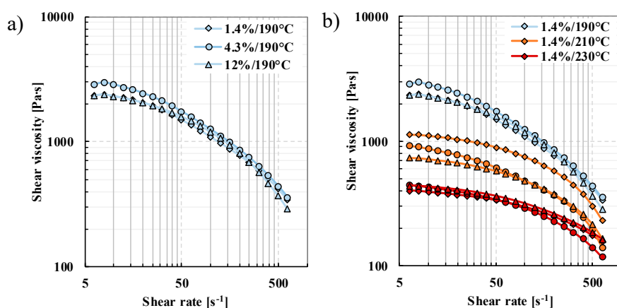
Figure 2. Shear viscosity of Ingeo 4032D (1.4%), 2003D (4.3%), and 4060D (12.0%) PLA (a) different D-lactide contents at 190 °C, (b) different temperatures (190 °C, 210 °C, and 230 °C).
