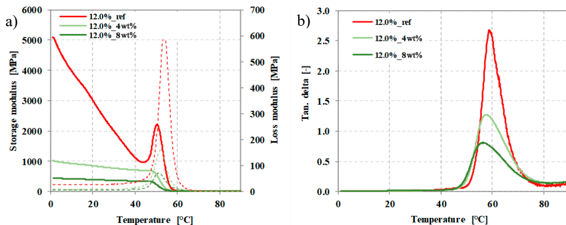
Figure 13. (a) Storage and loss moduli, (b) \tan\delta of the produced sheet foams as a function of temperature.
