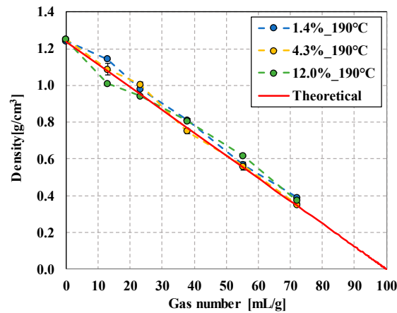
Figure 7. The density of samples prepared at 190 °C as a function of the gas number (theoretically calculated density is shown with a red line).
