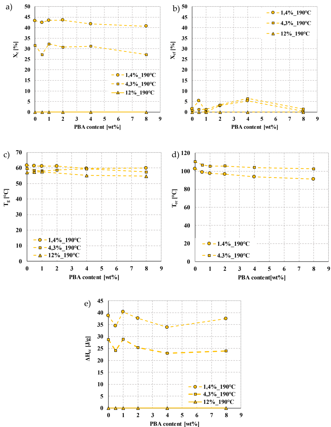
Figure 10. DSC (1st heating) results of foams produced from three types of PLAs with different D-lactide contents (a) crystalline fraction, (b) crystalline fraction during processing, (c) glass transition temperature, (d) cold crystallization temperature, (e) cold crystallization enthalpy at a processing temperature of 190 °C.
