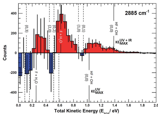
Fig. 5 Total kinetic energy ( E_{\text{TOT}} = \text{eKE} + \text{KER} ) difference (IR–no-IR) spectra for \text{IR} = 2885 \text{ cm}^{-1} , showing IR-excited (top) and no-IR (bottom) energetic limits. Blue and red areas indicate suppression and enhancement, respectively, relative to the no-IR spectrum. Error bars correspond to \sqrt{N_{\text{IR}} + N_{\text{no-IR}}} for each bin.
