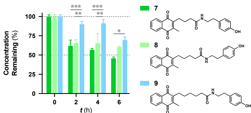
Figure 2. Comparison of metabolic stability and carbon chain length between the quinone core and the amide linkage for the structurally similar tyramine derivatives 7–9. Data was expressed as mean \pm SEM from at least one experiment, with at least three data points each: *** p < 0.001 , ** p < 0.002 , * p < 0.033 .
