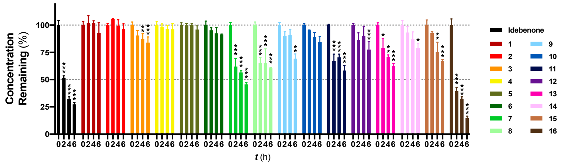
Figure 1. Metabolic stability study of 16 new SCQs and the reference benzoquinone idebenone. HepG2 cells were exposed to each SCQ at 40 \mu M for up to 6 h. Concentrations found at t = 0 were normalized to 100% and concentrations found at other time points were normalized by accordingly dividing by the concentrations found at t = 0 , \times 100\% . Data was expressed as mean \pm standard error of mean (SEM) from at least one experiment, with at least three data points each. Two-way ANOVA was performed to compare concentrations found at t = 2 h, 4 h, 6 h to t = 0 for each compound: *** p < 0.001 , ** p < 0.002 , * p < 0.033 .
