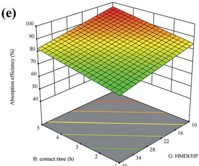
Fig. 13 Interaction of factors with the rate of adsorption efficiency.
