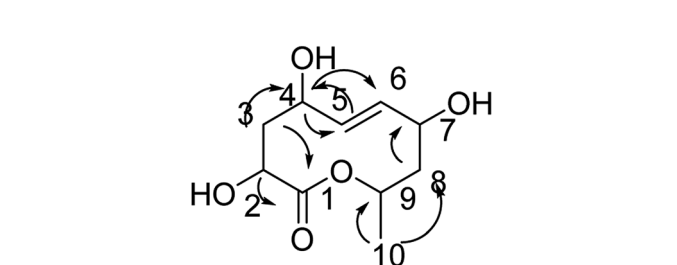
Fig. 9 The key HMBC correlations of compound 8.
