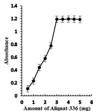
Fig. 3 The effect of the amount of Aliquat-336 (mg) on the optical sensor response of BTMP with 1.0 \times 10^{-5} M of \text{Ag}^+ .
