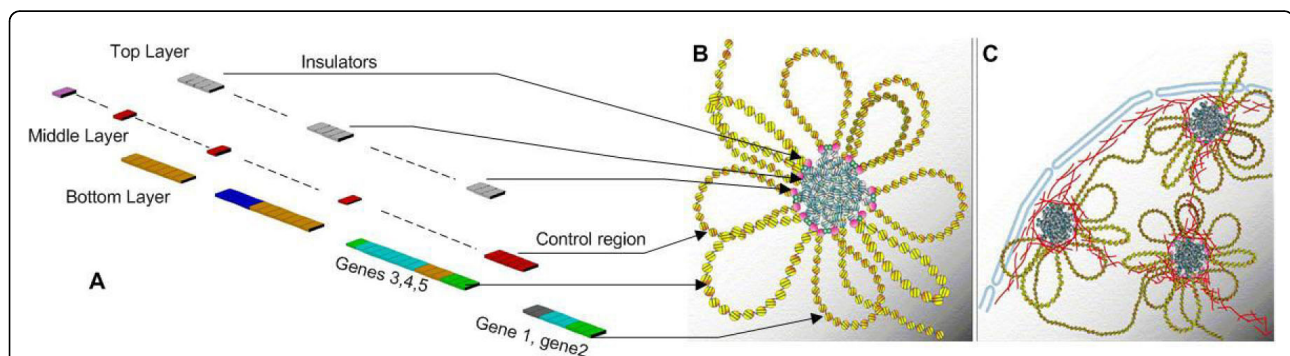
Figure 4 Organized cluster mapping of DNA to Nucleus. Mapping of DNA strand into DNA Hard Drive: A) shows the DNA strand decomposed into its information structure. The top layer (gray) contain the strategic placement of insulators, the middle layer contains the regulatory control regions (red) that controls the copy process of the genes and the bottom layer contains the genes organized into a form that allows co-expression. B) Shows the mapping of the insulators to the nuclear lamin substrate to form insulator clusters. These cluster are placed such that they structurally partition the genes into organized clusters. The regulatory control regions (red) now become specific to the rosette pattern formed from the insulator clusters. This results in a rosette pattern of genes and their control regions. C) Shows the placement of the rosette patterns to the nuclear lamin substrate within the nucleus thus creating the DNA hard drive. The red lines indicate the lamin. Pictures B and C from Maya, Corces, Capelson and Victor, "Biology of the cell" with permission. Available online 09 September 2004.
