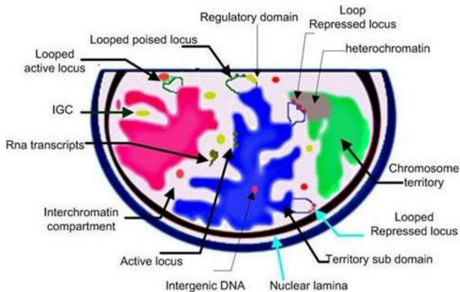
Figure 3 DNA organization. (redrawn from Kosak and Groudine, 2004). Architecture of DNA organization within the nucleus. Current view of how active genes are positioned in the nucleus and silenced genes are compartmentalized.
