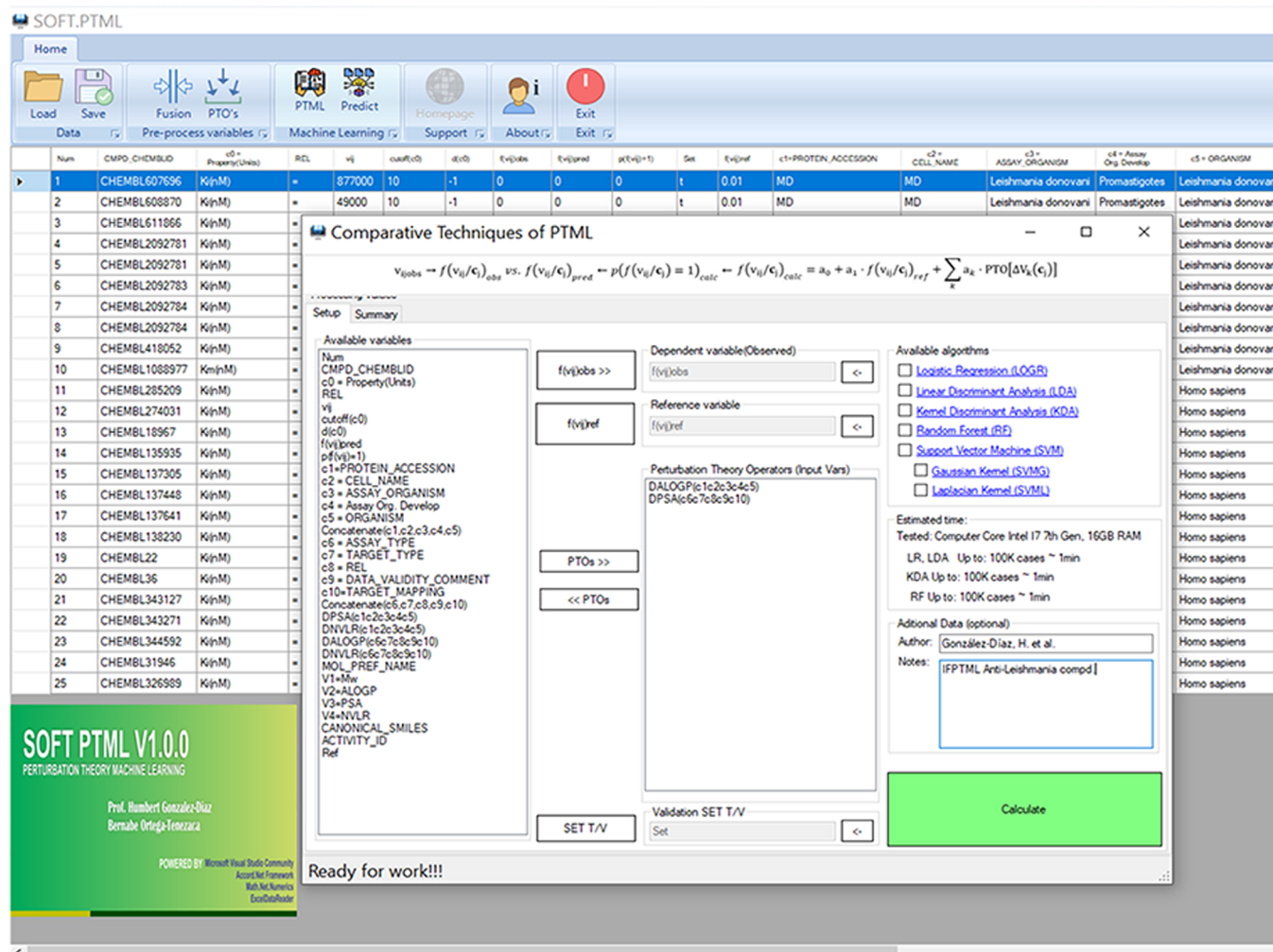
Figure 4. SOFT.PTML interface for analysis of ChEMBL antileishmanial compounds data.
