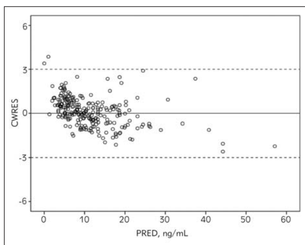
Figure 1 Diagnostic plot conditional weighted residuals (CWRES) versus population predictions (PRED) for the final model.
