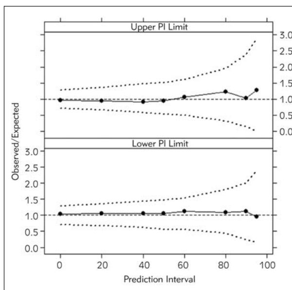
Figure 2 Numerical predictive check of the final population model for sirolimus. Circles present lower and upper limits of prediction intervals (%) observed in the data. Dashed lines indicate 95% CIs of the lower and upper limits of simulation-based prediction intervals (%).
