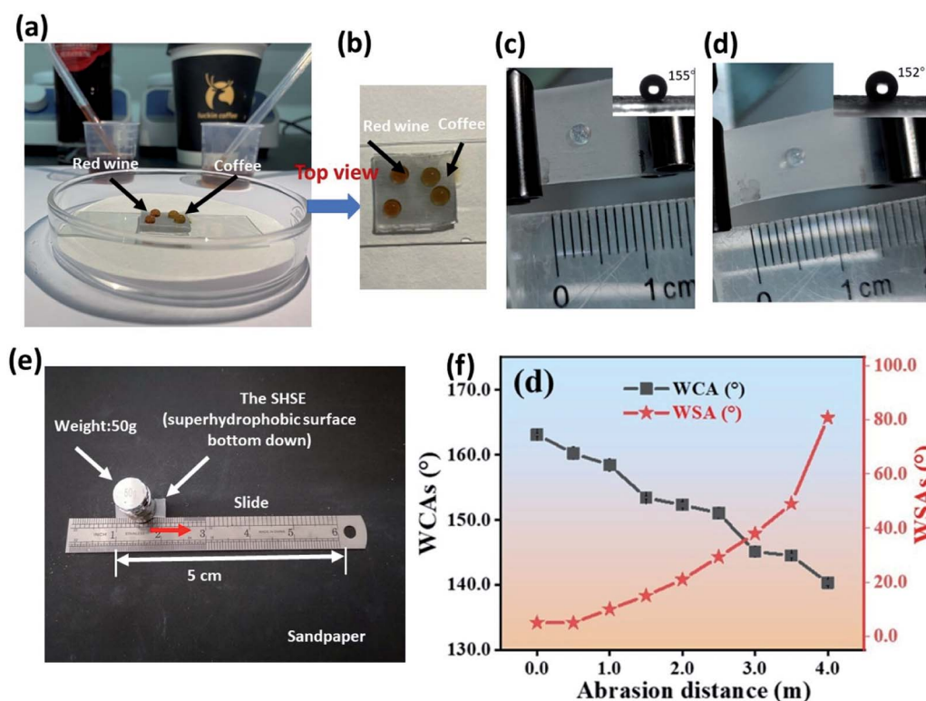
Fig. 6 (a) Side view and (b) top view images of the superhydrophobic effect proved by red wine and coffee; superhydrophobicity test (c) before and (d) after stretching to 130%; (e) schematic diagram of sandpaper abrasion test. (f) WCAs and WSAs after each abrasion test.
