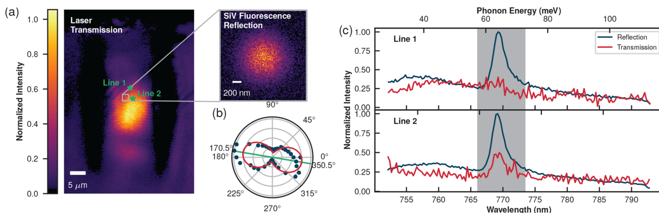
Figure 2. Device characterization. (a) Confocal scan (detected in transmission) of the waveguide, to map the waveguide mode. The laser wavelength is set to 738 nm and the polarization is set to the polarization of the waveguide. The inset shows a confocal scan of the SiV center in reflection at resonance ( \lambda = 739.338 nm) and the markings reveal the position of the defect center within the waveguide. Also, the green stars mark the positions of Line 1 and 2. (b) Polarization dependence of the waveguide, measured in the same configuration as in part (a), but the laser is placed at the waveguide mode maximum. (c) Spectrum of the PSB for the PLE measurement for two different and spatially separated transitions, Line 1 at 738.404 nm and Line 2 at 738.327 nm, normalized in transmission to the reflection spectrum. The gray shaded area denotes the local mode at 64 meV.
