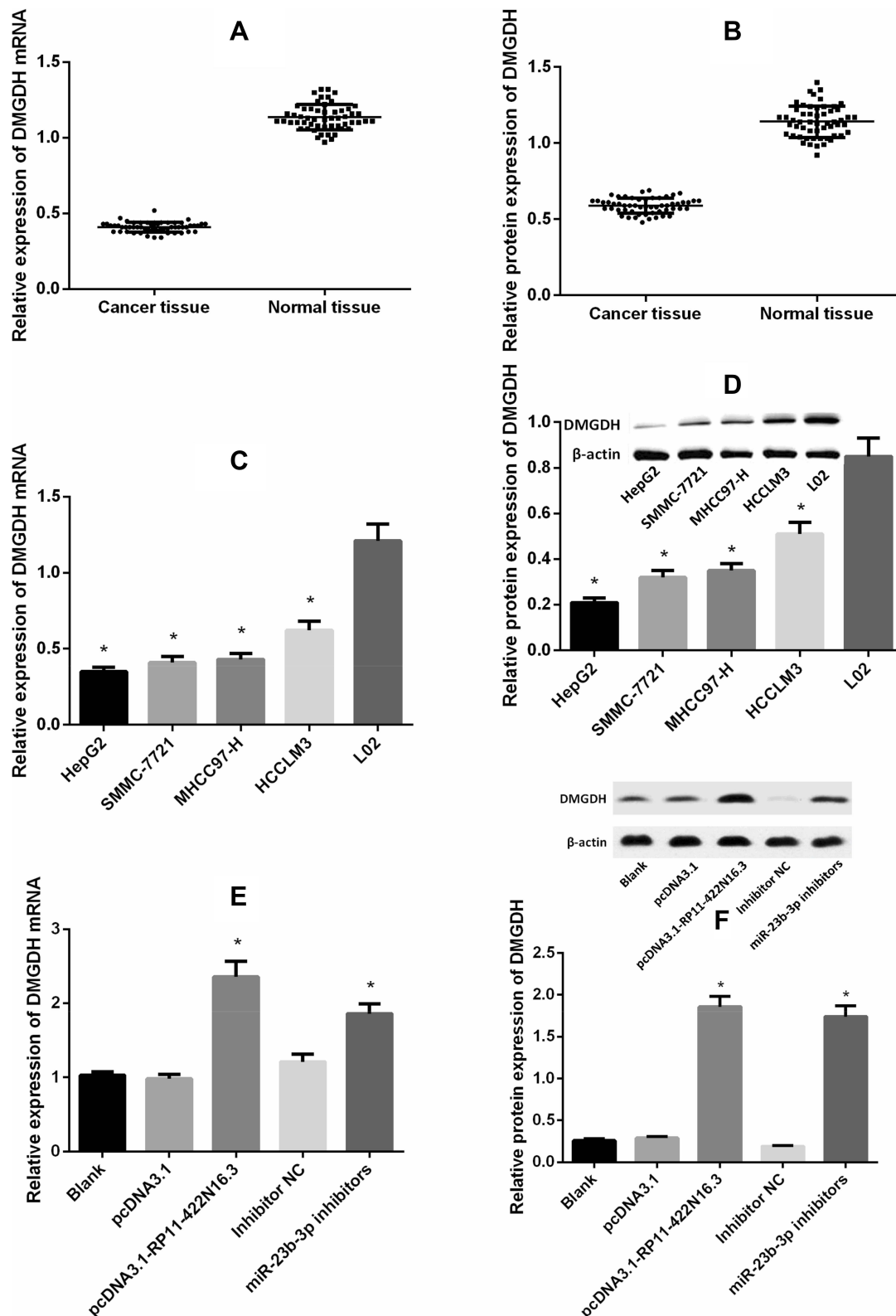
Figure 8 DMGDH expression in cancer tissue and normal tissue (( A ): DMGDH mRNA expression; ( B ): DMGDH protein expression), and in hepatocellular carcinoma cell lines (HepG2, SMMC-7721, MHC97-H and HCCLM3) and normal liver cell line (L02) (( C ): DMGDH mRNA expression; ( D ): DMGDH protein expression). Effect of RPI1-422N16.3 and miR-23b-3p on DMGDH expression (( E ): DMGDH mRNA expression; ( F ): DMGDH protein expression). *Indicated that P < 0.05 compared to Blank or L02 groups.
