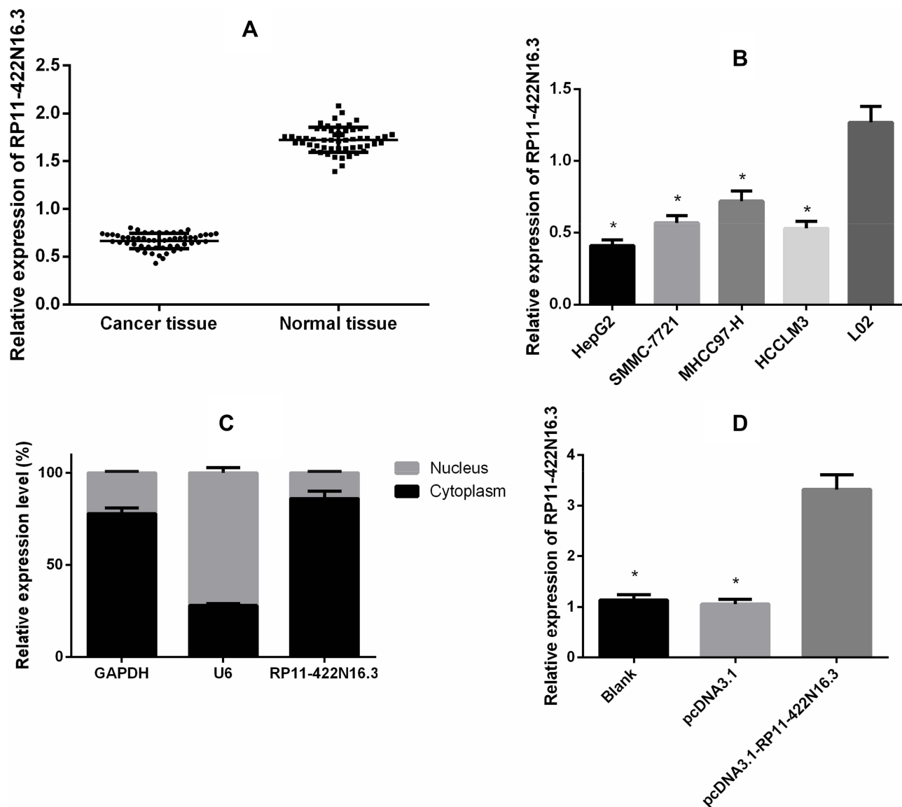
Figure 1 RP11-422N16.3 expressions in liver cancer tissue and cell lines. (A): relative RP11-422N16.3 expression in normal tissues and cancer tissues; (B): Relative RP11-422N16.3 expression in hepatocellular carcinoma cell lines (HepG2, SMMC-7721, MHCC97-H, and HCCLM3) and normal live cell line (L02); (C): RP11-422N16.3 expression in cytoplasm was higher than that in nucleus in subcellular fractionations; (D): overexpression of RP11-422N16.3 in HepG2 cell was successfully established. *Indicated that P < 0.05 compared to L02 or Blank group.
