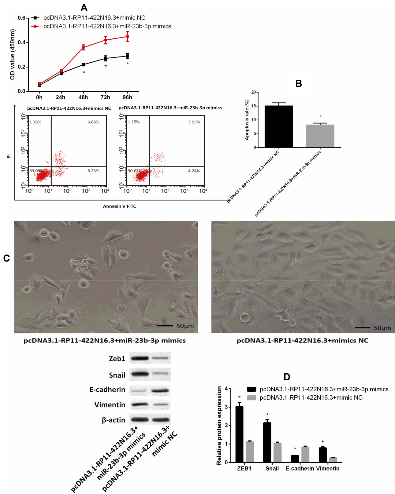
Figure 7 Mir-23b-3p reversed the effect of RP11-422N16.3 on cell proliferation (A) and cell apoptosis (B). Observation of cell morphology showed that HepG2 cells co-transfected with pcDNA3.1-RP11-422N16.3 and miR-23b-3p mimics changed to fusiform shape similar to mesenchymal cells (C). miR-23b-3p reversed the effect of RP11-422N16.3 on EMT-related biomarker expressions (D). *Indicated that P < 0.05 compared to pcDNA3.1-RP11-422N16.3+mimic NC group.
