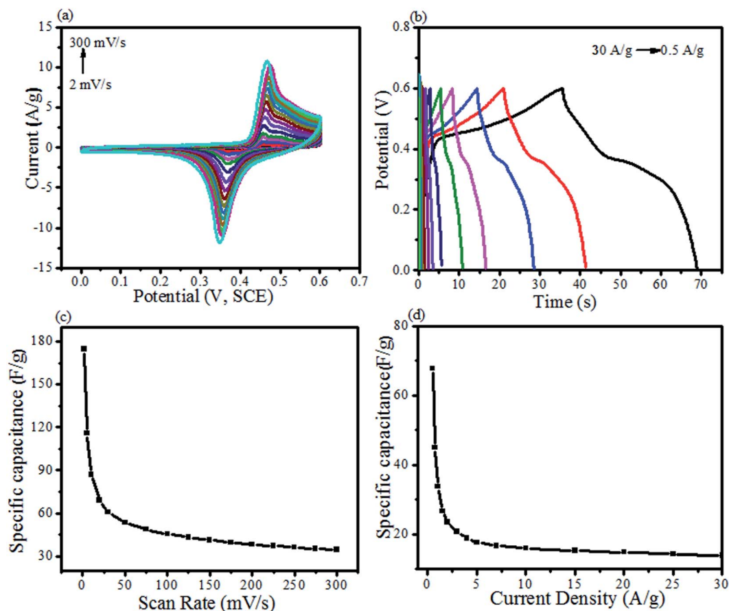
Fig. 8 Supercapacitive properties of the ZnO@PdO/Pd electrode by (a) CV at applied scan rates (ASR), (b) GCD measurements at applied CD, (c) SC of ZnO@PdO/Pd electrode at ASR, and (d) SC at applied CD.
