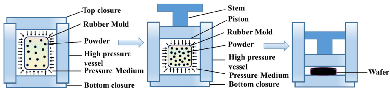
Fig. 6 Isostatic-pressing method.
