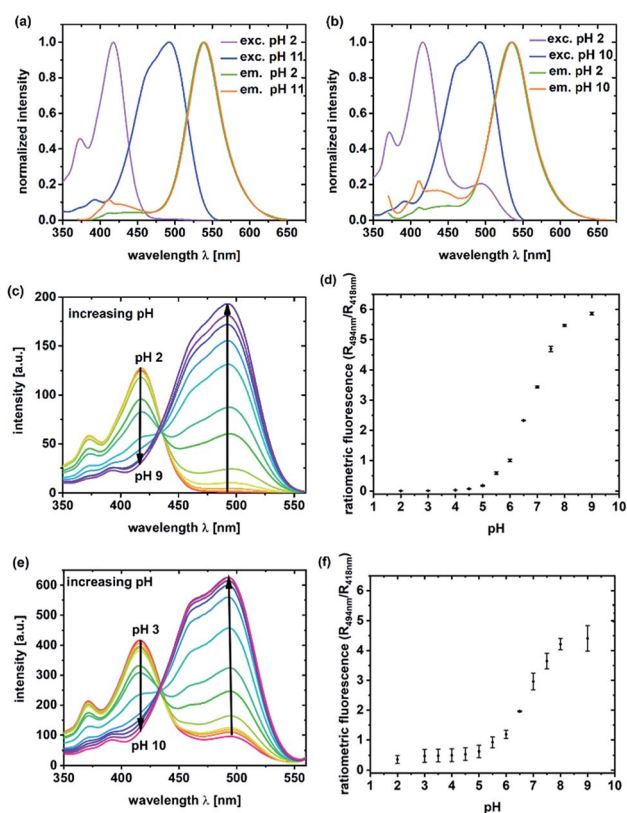
Fig. 1 Excitation (exc.) ( \lambda_{\text{em}} = 570 \text{ nm} ) and emission spectra (em.) ( \lambda_{\text{exc}} = 360 \text{ nm} ) of C-NP (a) and CS-NP (b) at \text{pH} 2 (ROH) and 11 or 10 , respectively (RO - ); excitation titration ( \lambda_{\text{det}} = 570 \text{ nm} ) of C-NP (c) and CS-NP (e) at various \text{pH} values. The corresponding fluorescence intensity ratios are shown in (d) and (f) and are averaged over three independent measurements.
