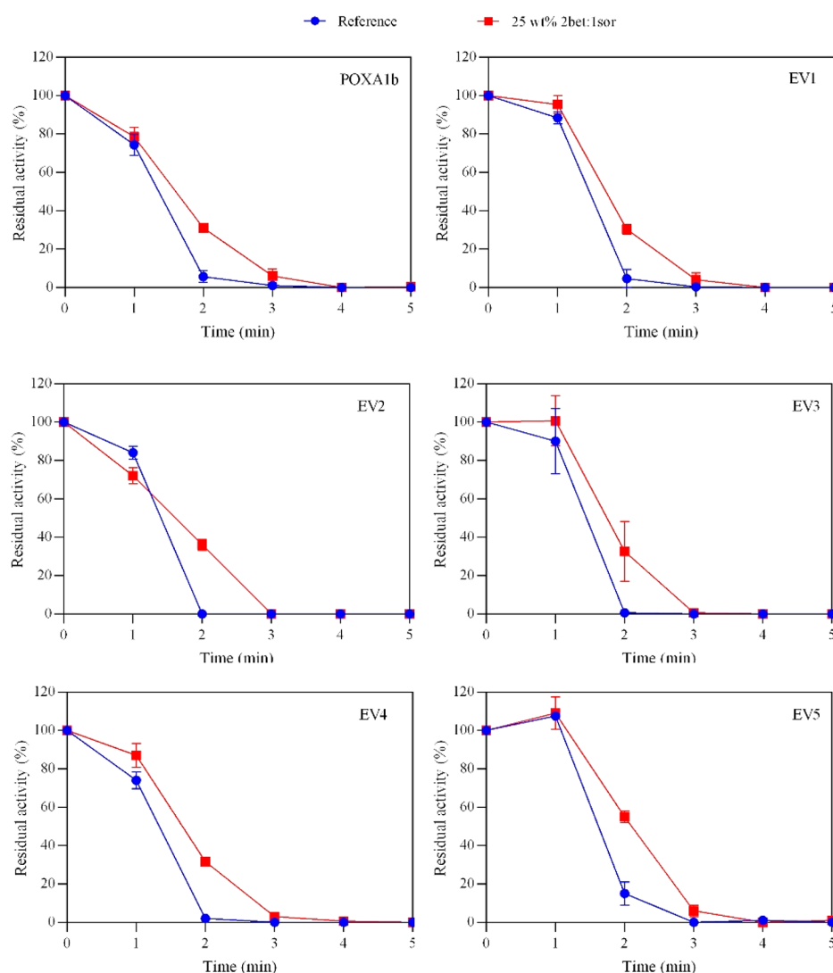
Figure 6. Comparison of thermostability of 1.25 g L -1 laccases in 50 mM phosphate buffer, pH 7 aqueous solution in the absence (blue dots), and in the presence of 25 wt % of 2Bet:1Sor (red squares) at 90 °C. The residual activity (%) is determined by comparing the activity measured after a set amount of time with the free-DES phosphate buffer, pH 7.0 and 50 mM at 25 °C (reference, 100%).
