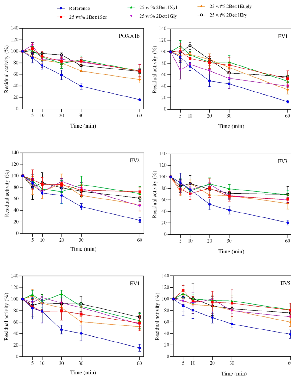
Figure 1. Comparison of thermostability of 1.25 \text{ g L}^{-1} laccases in 50 mM phosphate buffer, pH 7 aqueous solution in the absence (blue dots), and in the presence of 25 wt % of 2Bet:1Sor (red squares), 2Bet:1Xyl (green triangles), 2Bet:1Gly (purple triangles), 2Bet:1Et.gly (orange dots), and 2Bet:1Ery (black circles) at 70 °C. The residual activity (%) is determined by comparing the activity measured after a set amount of time with the free-NADES phosphate buffer, pH 7.0 and 50 mM at 25 °C (reference, 100%).
