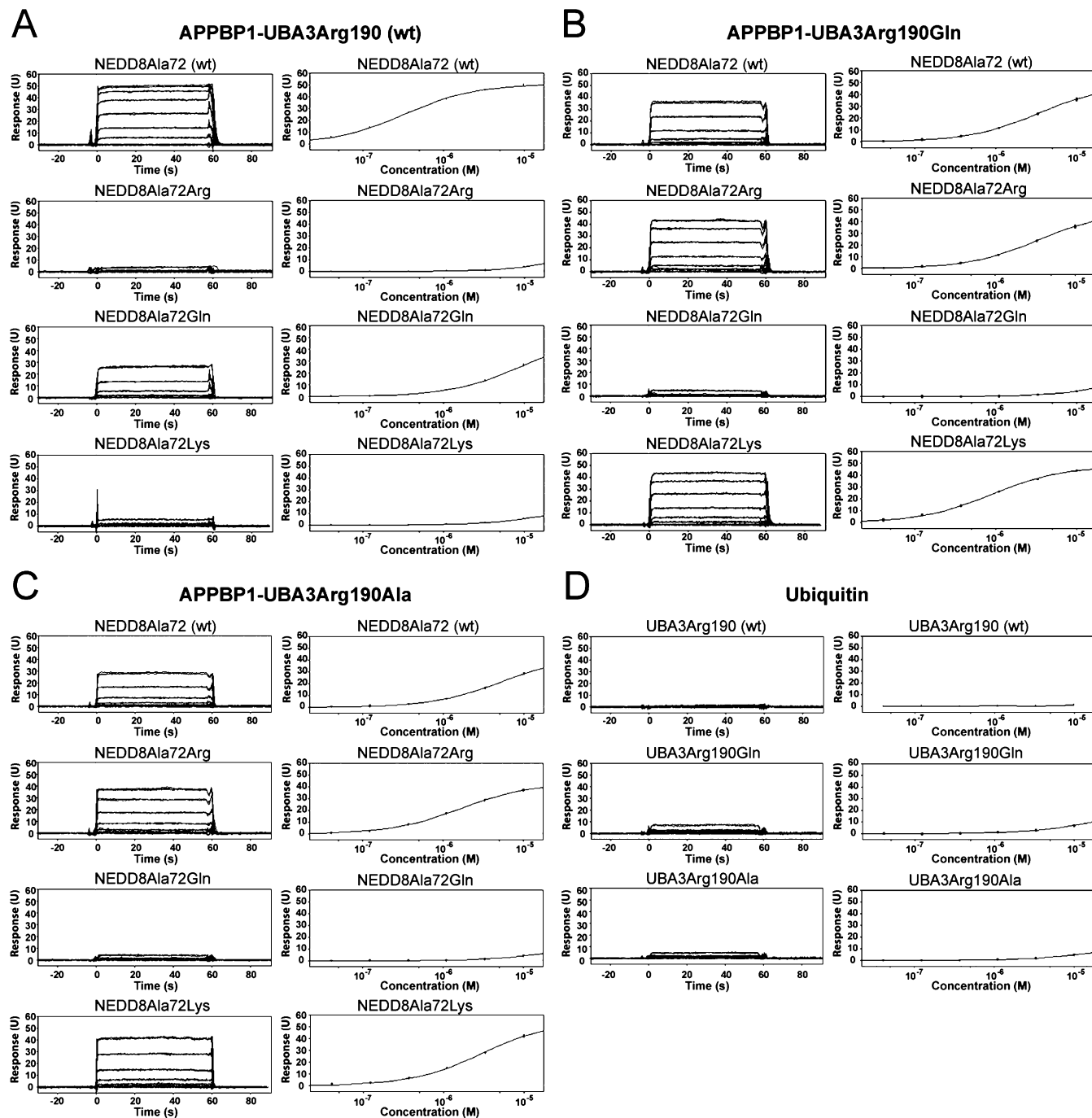
FIGURE 2: Surface plasmon resonance analysis of APPBP1-UBA3 binding to UBLs. Representative sensorgrams (left) and binding curves (right) from surface plasmon resonance interaction assays, performed as described in Experimental Procedures, for (A) GST-APPBP1-UBA3Arg190 (wt), (B) GST-APPBP1-UBA3Arg190Gln, and (C) GST-APPBP1-UBA3Arg190Ala with NEDD8Ala72 (wt), NEDD8Ala72Arg, NEDD8Ala72Gln, and NEDD8Ala72Lys, as indicated. (D) Representative sensorgrams (left) and binding curves (right) for ubiquitin binding to GST-APPBP1-UBA3Arg190 (wt), GST-APPBP1-UBA3Arg190Gln, and GST-APPBP1-UBA3Arg190Ala, as indicated.
