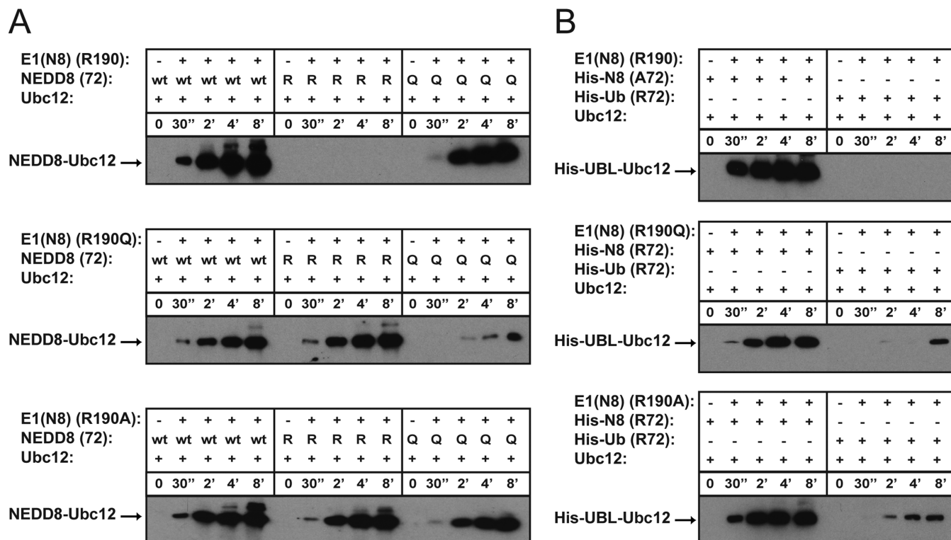
FIGURE 3: Altered E1 NEDD8 (APPBP1-UBA3)-E2 (Ubc12) transthiolation specificity for UBA3 Arg190 mutants. (A) Time-course of forming the Ubc12–NEDD8 thioester complexes with 100 nM wild-type and indicated mutants of APPBP1-UBA3, 4 \mu M wild-type and indicated mutants of NEDD8, and 3 \mu M Ubc12. Reactions were stopped at the indicated times, products were separated by SDS–PAGE and detected by Western blotting with anti-NEDD8 antibodies. (B) Western blots of reactions performed as in panel A, except using the indicated His-NEDD8 variants and His-ubiquitin, and probed with anti-His-tag antibodies.
