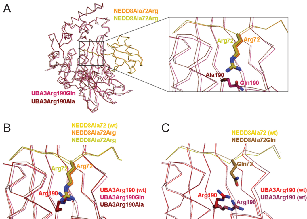
FIGURE 4: Structural basis for UBA3's Arg190s negative selectivity against a UBL's Arg72. Superimposition of wild-type (2I) and mutant APPBP1-UBA3-NEDD8 structures was performed using least-squares fitting over all atoms in O (33). UBA3's residue 190 is shown in various shades of red; NEDD8's residue 72 in yellow; nitrogen, blue; and oxygen, light red. (A) Overall superimposition of APPBP1-UBA3Arg190Gln (rose)-NEDD8Ala72Arg (melon, "ubiquitinated") and APPBP1-UBA3Arg190Ala (maroon)-NEDD8Ala72Arg (chartreuse, "wild-type-opposite") complexes, with close-up view around the NEDD8 mutant's Arg72 and UBA3's residue 190. (B) Close-up view showing NEDD8 mutant Arg72 from APPBP1-UBA3Arg190Gln-NEDD8Ala72Arg (melon) and from APPBP1-UBA3Arg190Ala-NEDD8Ala72Arg (chartreuse), and Arg190 (red) from wild-type APPBP1-UBA3-NEDD8. (C) Close-up view showing Arg190 (violet) and NEDD8 mutant Gln72 from APPBP1-UBA3Arg190 (wt)-NEDD8Ala72Gln, and Arg190 (red) from wild-type APPBP1-UBA3-NEDD8.
