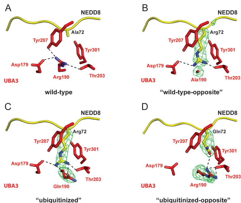
FIGURE 5: Differential APPBP1-UBA3 interactions with NEDD8 for UBA3 residue 190 and NEDD8 residue 72 mutants. Stick-representation close-up views, with UBA3 colored red and NEDD8 colored yellow, nitrogen blue, oxygen light-red, and hydrogen bonds shown as dashed lines for (A) APPBP1-UBA3-NEDD8 (wild-type), (B) APPBP1-UBA3Arg190Ala-NEDD8Ala72Arg (“wild-type-opposite”), (C) APPBP1-UBA3Arg190Gln-NEDD8Ala72Arg (“ubiquitimized”), and (D) APPBP1-UBA3Arg190 (wt)-NEDD8Ala72Gln (“ubiquitimized-opposite”) complexes. Simulated annealing omit F_o - F_c electron density maps are shown in green mesh, contoured at 3\sigma over UBA3’s residue 190 and NEDD8’s residue 72 in panels B–D. The maps were calculated using the program CNS (32), after simulated annealing at 2000 K omitting both UBA3’s residue 190 and NEDD8’s residue 72.
