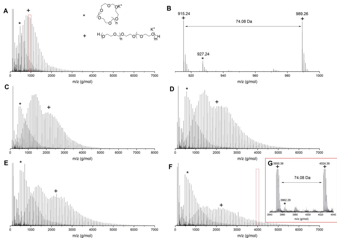
Fig. 3 MALDI-ToF spectrum (reflection mode) for polymerization 1 in Table 1 at different conversions (A) 6% conversion, (B) zoom in of 6% conversion, (C) 19% conversion, (D) 25% conversion, (E) 37% conversion and (F) 65% conversion (G) zoom in of 65% conversion. Linear polymer (C_3H_6O_2)_n C_2H_6O_2 K (+); cyclic polymer (C_3H_6O_2)_n K (*).
