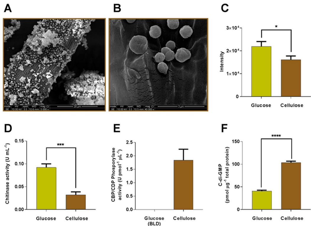
Figure 1. Changes in morphology, enzymatic and metabolite profile of F. succinogenes S85 during growth on cellulose. Scanning electron microscopy of F. succinogenes S85 cells attached to microcrystalline cellulose. Images showed adherence of cells to microcrystalline cellulose particles. Parallel grooves and pits have been left behind in places where cells have detached from the cellulose particle ( A and B ). Scanning densitometry of O-antigen carbohydrate moiety of LPS obtained from F. succinogenes S85 cells grown in glucose and cellulose substrate. Results are an average of three biological replicates ( C ). Chitinase activity of F. succinogenes S85 on cellulose vs glucose-grown cells. Results are an average of two biological replicates and two technical replicates ( D ). Cellobiose/celldextrin phosphorylase activity of F. succinogenes S85 on cellulose vs glucose-grown cells. Results are an average of three biological replicates and three technical replicates. In glucose cellobiose/celldextrin phosphorylase activity was below the limit of detection (BLD) ( E ). Quantification of cyclic-di-GMP (c-di-GMP) in response to cellulose and glucose. Results are an average of two biological and two technical replicates ( F ). Error bars indicate standard deviation and stars indicate the level of significance between conditions as determined using two-tailed Student's t test at 95% confidence. p -value less than 0.05 and greater than 0.01 is represented by *, p -value less than 0.01 but greater than 0.001 is represented by **, p -value less than 0.001 but greater than 0.0001 is represented by *** and p -value less than 0.0001 is represented by ****.
