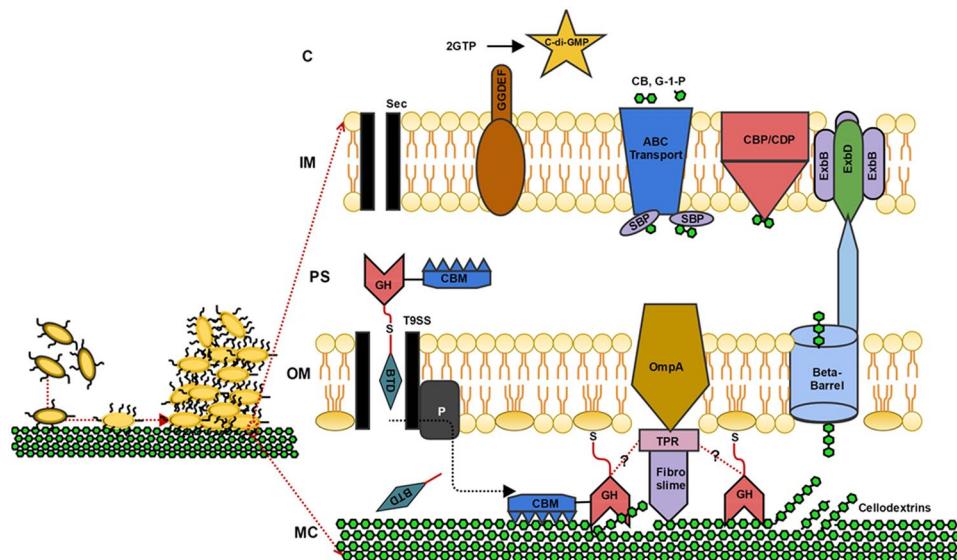
Figure 2. Proposed model of the mechanism of cellulose metabolism in F. succinogenes S85. Bacterial attachment to MC cellulose is the first step during lignocellulose degradation. Translocation of cellulases to the surface occurs using T9ss-dependent pathway. On the cell surface, cellulases are attached to Lipid A at the outer membrane via serine residues and form a multi-protein complex along with OmpA, TPR and fibroslime proteins. Released products of cellulolysis (cellodextrins) are then imported to the periplasm via beta barrel proteins and the TonB/ExbB/ExbD active transport system. Cellodextrin phosphorylases cleave cellodextrin into glucose-1-phosphate and cellobiose at the periplasmic side of cytoplasmic membrane, which are then transported to the cytoplasm via the concerted action of solute binding proteins and ABC transporters. CBM ; carbohydrate binding modules, GH ; glycosyl hydrolase (figure depicts two GHs as a representative example of the presence of GHs in the multiprotein complex), BTD ; basic terminal domain, OmpA ; outer membrane protein A, TPR ; tetratricopeptide repeats, CBP/CDP ; cellobiose/cellodextrin phosphorylase, SBP ; solute binding proteins, CB ; cellobiose, G-1-P ; glucose-1-phosphate, GGDEF ; diguanylate cyclase domain, GTP ; guanosine triphosphate, C-di-GMP ; cyclic di guanosine monophosphate, ABC ; ATP-binding cassette transporters, T9ss ; Type IX secretion system, ExbB/ExbD ; biopolymer transport proteins, MC ; microcrystalline cellulose, OM ; outer membrane, IM ; inner membrane, PS ; periplasmic space, C ; cytoplasm, SEC ; secretion pathway, P ; peptidase.
