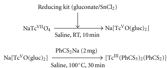
FIGURE 2: Synthesis of ^{99\text{m}}\text{Tc} -SSS.
