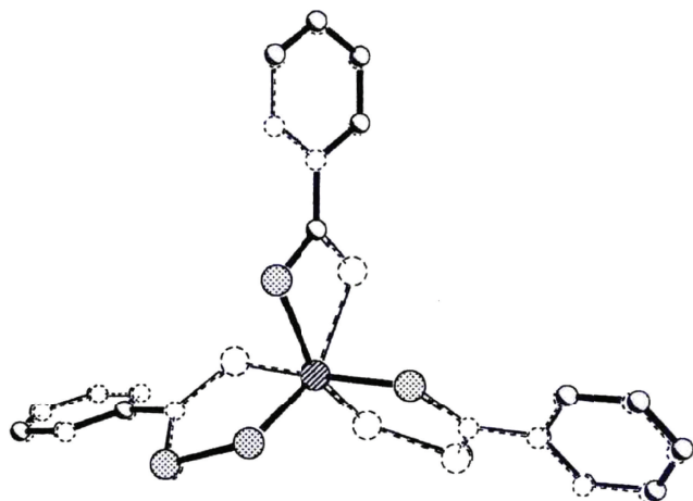
FIGURE 1: Superposition of the crystal structures of ^{185/187}\text{Re} -SSS and ^{99}\text{Tc} -SSS complexes (reprinted from: N. Lepareur, Ph.D. thesis no. 2003 REN 10110, 2003).
