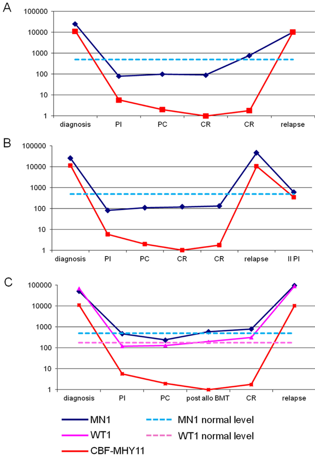
Figure 3: Panel A and B: MN1 transcript expressed as number of copies/10 4 ABL copies (blue line) and CBFβ-MYH11 transcript expressed as copy number/10 4 ABL copies (red line) at diagnosis and during follow-up in two patients with inv(16) who relapsed. MN1 increased above the upper normal limit three months before relapse in patient represented in panel A. Panel C: MN1 transcript (blue line), CBFβ-MYH11 transcript (red line) and WT1 transcript (pink line) at diagnosis and during follow-up of a patient with an inv(16) alteration who relapsed after two cycles of chemotherapy and allogeneic bone marrow transplantation (allo BMT). MN1 and WT1 increased above the upper normal limit four months before haematological relapse. PI= post induction, PC= post consolidation, CR= complete remission.
