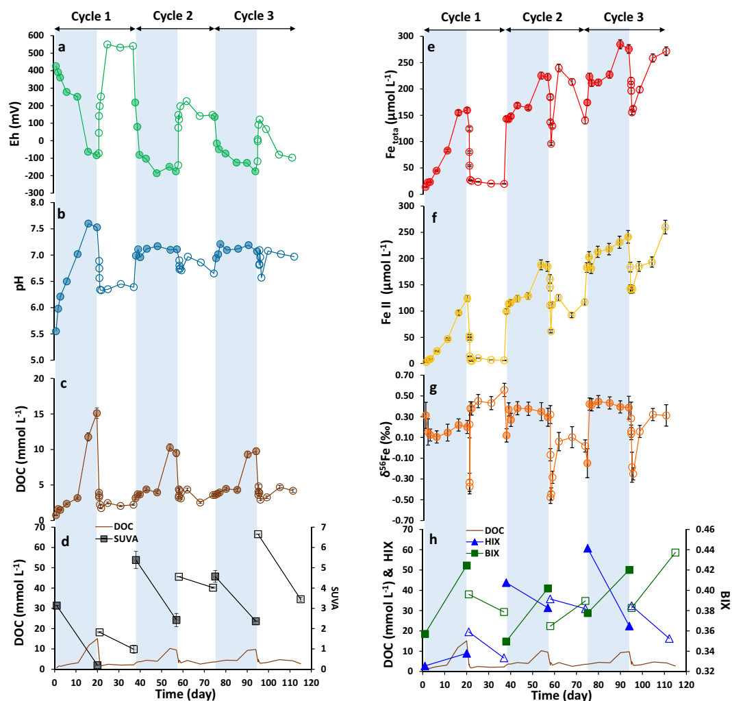
Figure 1. Evolution of Eh (a), pH (b), DOC (c), SUVA (d), Fe_{tot} (e), Fe(II) (f), \delta^{56}Fe (g) and the BIX and HIX indexes (h) versus time (day) during the anoxic/oxic cycles. Eh and pH were measured in the soil suspension and other parameters were determined in filtrates of 0.2 \mu m . The blue zones illustrate the anoxic periods and the white ones the oxic periods. The filled and empty symbols correspond to samples under anoxic and oxic conditions, respectively. Analytical error bars were calculated by (i) measuring the standard for DOC, Fe(II) Fe_{tot} , and \delta^{56}Fe (2SD) analyses, (ii) average of Replicates analyses ( n=2 or 3) for SUVA, and (iii) Eq. (3) if there were replicates of analysis.
