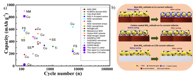
Fig. 7 (a) Comparison of cycling performance of previous \text{NiS}_2 reports (Cu: copper; FS: free-standing; Ti: titanium; NM: not mentioned; C/Al: carbon-coated aluminium current collectors, respectively), where circles indicate carbonate electrolyte and squares indicate ether electrolyte. (b) Schematic diagram illustrating the mechanism of side reactions involving the current collector.
