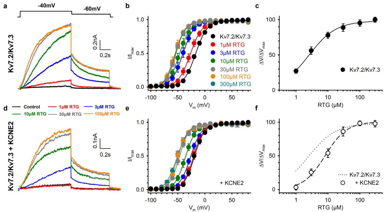
Figure 1. KCNE2 decreases the retigabine sensitivity of heterotetrameric K_v7.2 - K_v7.3 channels. (a) Effect of increasing concentrations of retigabine (1–100 \mu\text{M} ) on K_v7.2 - K_v7.3 currents. Retigabine potentiated the K_v7.2 - K_v7.3 current in a concentration-dependent manner, and saturation occurred above 30 \mu\text{M} . Voltage protocol is shown on top. (b) Voltage-dependence of activation. Increasing concentrations of RTG caused a gradual hyperpolarizing shift. (c) Concentration-effect curve plotted as the shift in the voltage-dependence of activation normalized to the maximal observed shift ( \Delta V/\Delta V_{\text{max}} ) as function of the drug concentration. (d) Similar to (a) but after co-expression with KCNE2. Retigabine potentiated the K_v7.2 - K_v7.3 -KCNE2 currents but unlike (a) concentrations above 1 \mu\text{M} had to be used. (e) Voltage-dependence of activation. KCNE2 reduced the hyperpolarizing shift at every drug concentration, and decreased the maximal observed shift ( \Delta V_{\text{max}} ). (f) Concentration-effect curve.
