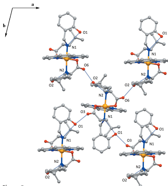
Figure 2 A view of the O–H \cdots O hydrogen bonds (dashed lines; see Table 1) in the crystal of compound I , forming layers that are parallel to the ab plane. All H atoms have been omitted for clarity.
