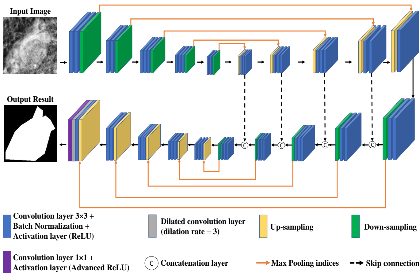
Figure 4. Architecture of the proposed Connected-SegNets model.
