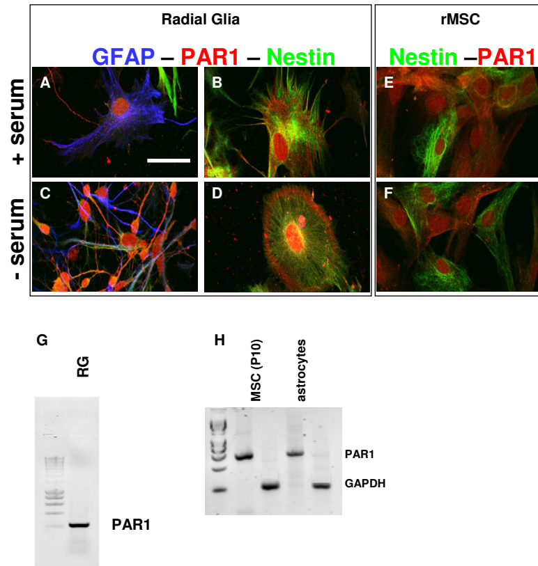
Expression of the PAR1 thrombin receptor in RG and rat MSCs cultures. RG and rat MSCs were cultured for 2 days in the presence of serum (A, B, E) or were maintained for the same time in serum-free medium (C, D, F). Then, the cells were fixed and RG were labelled with anti-nestin (green), anti-PAR1 (red) and anti-GFAP (blue) antibody (panel A-D) while rat MSCs were stained with anti-nestin (green) and anti-PAR1 (red) antibody (panel E, F). Scale bar (in A = 10 μm) applies to all images. Expression of thrombin receptor PAR1 mRNA in mouse RG (G) and rat MSCs and astrocytes (H) was analyzed by RT-PCR using optimized primers for each species.
