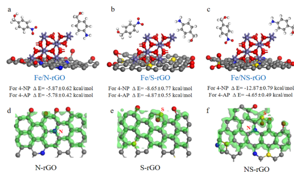
Fig. 8 (a–c) Calculated interaction energies among reactant (4-NP), product (4-AP), Fe/N-rGO, Fe/S-rGO and Fe/NS-rGO. Charge density differences of N-rGO (d), S-rGO (e) and NS-rGO (f).
