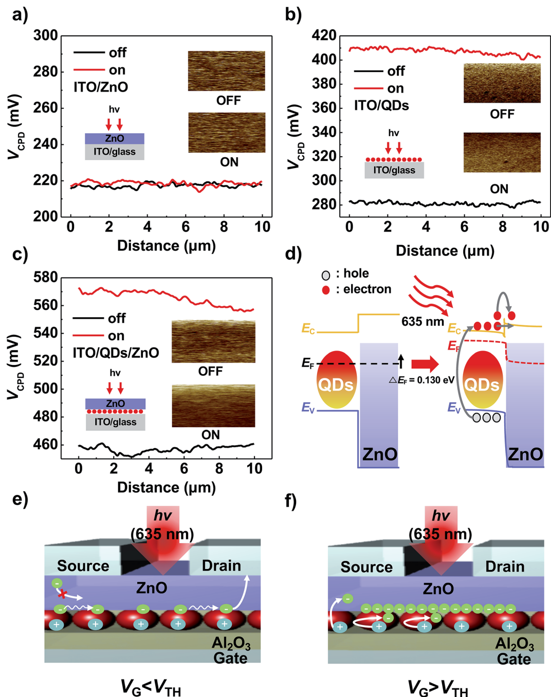
Fig. 6 V_{\text{CPD}} measurements of (a) ITO/ZnO and (b) ITO/QDs. (c) ITO/QDs/ZnO films with and without illumination at 635 nm. The topography profiles are shown in the insets. (d) Schematic interfacial energy band diagrams of the QDs and ZnO in darkness and during exposure to light. Schematic illustration of photocurrent channel formation in the device under illumination at \lambda = 635 nm when (e) V_{\text{G}} < V_{\text{TH}} (off state) and (f) V_{\text{G}} > V_{\text{TH}} (on state).
