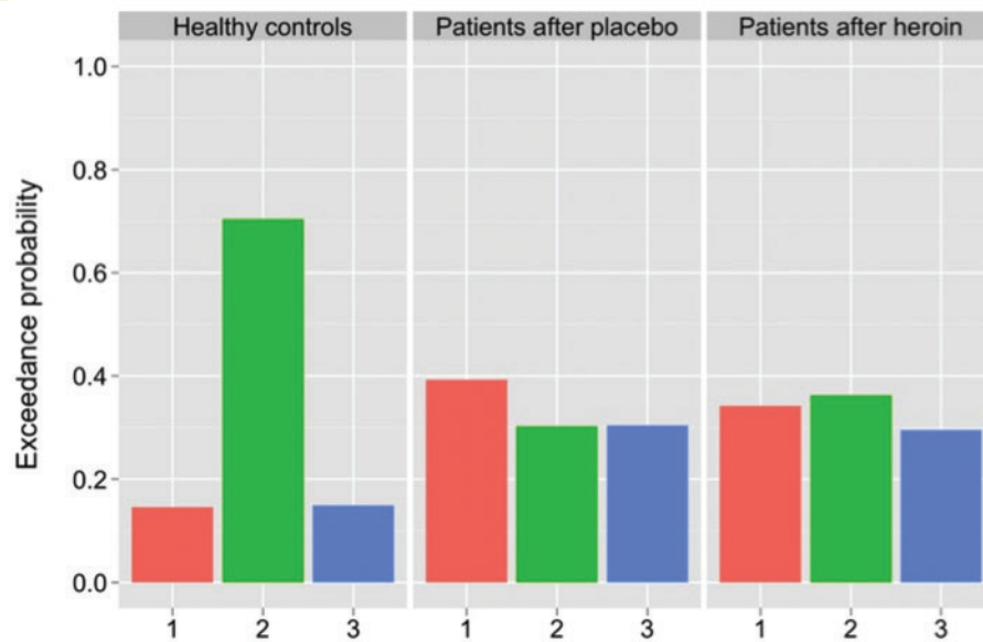
Figure 2 Bayesian model selection results. Bayesian model selection results among all three dynamic causal models. The models differed in whether they included fear-induced modulation of forward (Model 1), backward (Model 2) or both forward and backward connections (Model 3) among the visual-limbic-prefrontal network. Results for each treatment are expressed in terms of exceedance probability, the relative probability that this model is more likely than any other of the models tested, given the treatment data.
