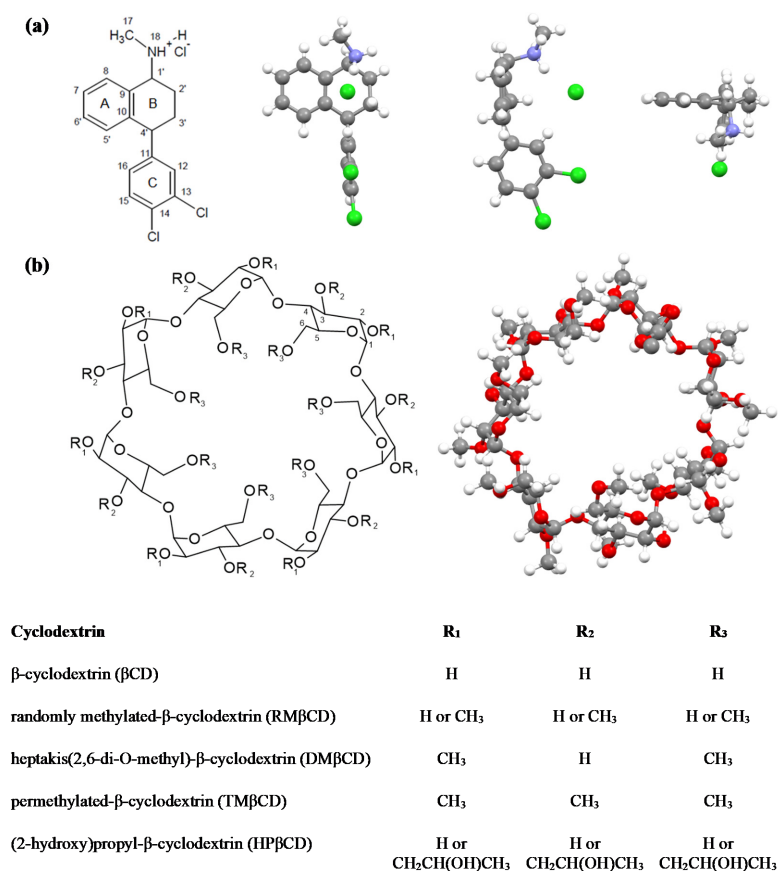
Figure 1. (a) Sertraline hydrochloride structural formula (on the left) and the models made based on crystal structure of sertraline hydrochloride (on the right) with refcode CAVVUQ [46] from the Cambridge Structural Database (CSD) [47] and (b) a general structural formula of some \beta -cyclodextrins (on the left) and crystal structure of RM \beta CD (on the right) with refcode JOSWOD [48] from the CSD [47].
