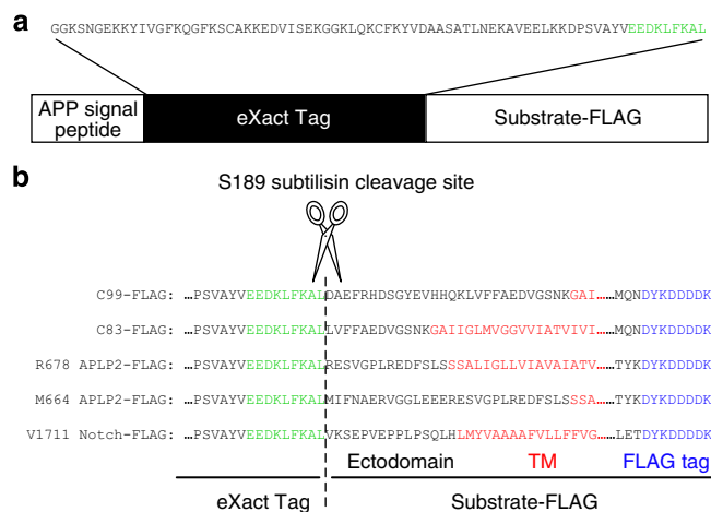
Figure 1 | Schematic diagrams of generating \gamma -secretase substrates.
