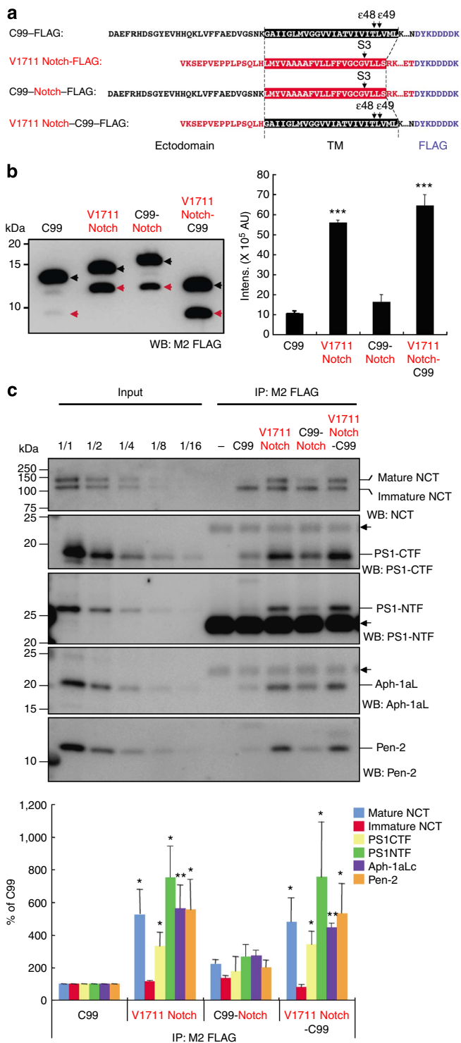
Figure 4 | Ectodomain swapping of C99 and V1711 Notch substrates.
