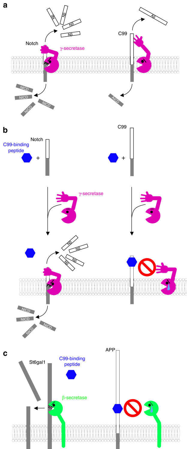
Figure 9 | Models for substrate preference of \gamma -secretase and inhibition of APP cleavage by C99-binding peptide.
