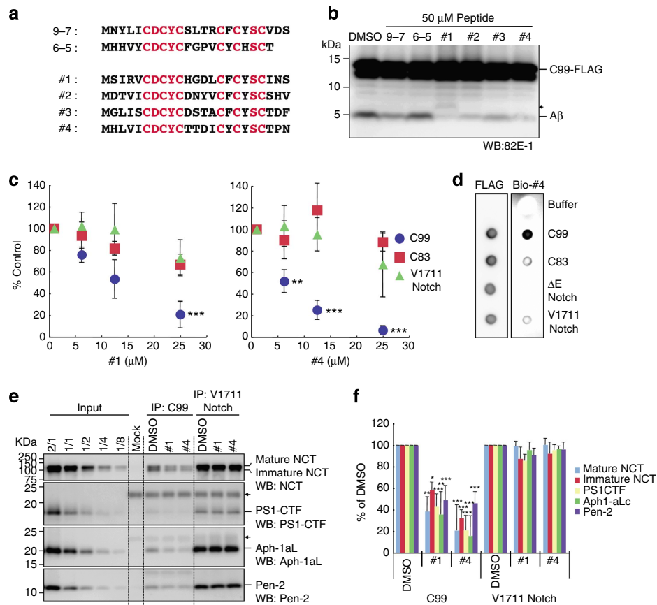
Figure 6 | Substrate-specific inhibition of \gamma -secretase-dependent C99 cleavage by C99-binding peptides. Peptide sequence of C99-binding peptides ( a ). Two peptides (9-7 and 6-5) were panned out using a cell-free peptide-displaying system. The CDCYCxxxxCxSC motif (in red) found in peptides 9-7 and 6-5 was used as a skeletal structure to generate 9-7 derivatives (peptides #1 to #4). C99-FLAG substrate was incubated with a CHAPSO-solubilized \gamma -secretase fraction in the presence of the peptides ( b ). These peptides inhibited A \beta production. The arrowhead indicates the retardation of A \beta migration caused by peptide #1. Peptides #1 and #4 specifically inhibited AICD production from C99-FLAG in a dose-dependent manner ( c ). Data are expressed as means \pm s.d. of three independent experiments. **P < 0.005 , ***P < 0.0005 (analysis of variance (ANOVA), Scheffe's post hoc test compared with DMSO control). Dot blot analysis of peptide #4 ( d ). Four picomols of substrates (C99-FLAG, C83-FLAG, V1711 Notch-FLAG and \Delta E Notch-FLAG) were placed on nitrocellulose and dehydrated. After blocking with 5% skim milk, the membrane was incubated with biotinylated peptide #4 and streptavidin-conjugated HRP and the peptide bound to the substrates was visualized. Peptide #4 selectively bound to the C99-FLAG. C99-FLAG or V1711 Notch-FLAG was immobilized using anti-FLAG M2 magnetic beads and mixed with a CHAPSO-solubilized \gamma -secretase fraction in the presence or absence of the peptides ( e ). Western blotting was used to visualize and quantify \gamma -secretase components in co-immunoprecipitates. The peptides significantly reduced the interaction of C99 with \gamma -secretase components compared with the interaction of V1711 Notch. Data are expressed as means \pm s.d. of three independent experiments ( f ). *P < 0.05 , **P < 0.005 , ***P < 0.0005 (ANOVA, Scheffe's post hoc test compared with DMSO control).
