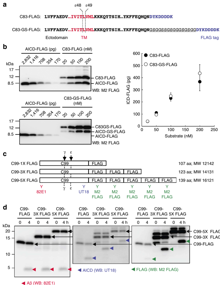
Figure 3 | Length of substrate C terminus is not critical for the cleavage efficiency. A GS-stretch (of 16-residues) was inserted prior to the FLAG tag to generate C83-GS-FLAG, a 99-residue substrate tagged FLAG sequence (equivalent in length to C99-FLAG) (a). C83-GS-FLAG was incubated with \gamma -secretase fraction and subjected to western blotting to visualize AICD-FLAG production (b). C83-GS-FLAG exhibited an indistinctive cleavage compared with C83-FLAG cleavage. Tandem repeats of FLAG tag were inserted at C99 C terminus to examine the effect of extension of intracellular domain length on cleavage efficiency (c). Attachment of tandem repeats of FLAG tags failed to alter production of A \beta and AICD (d).
