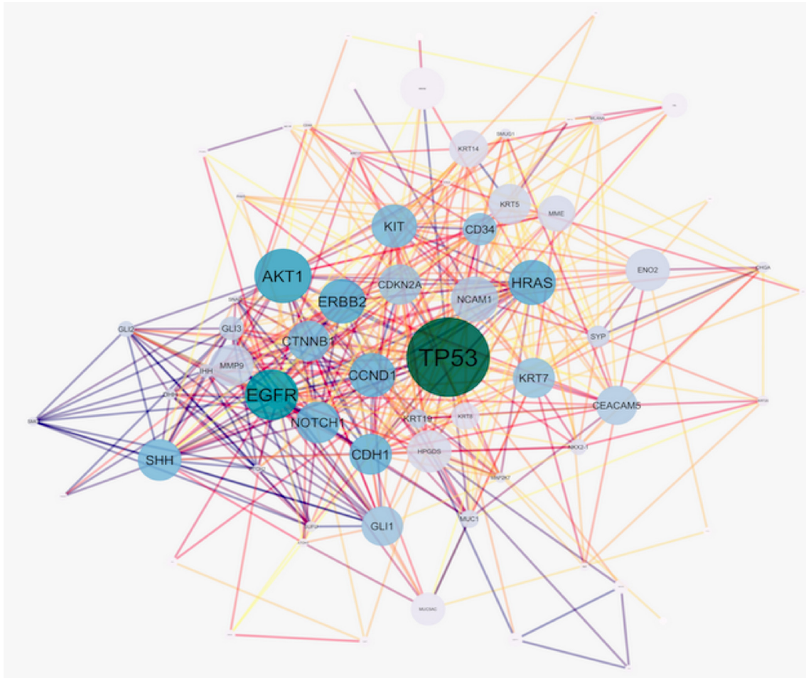
Figure1. The main connected component of skin carcinoma related network is shown. The network is layout based on degree (K) value and betweenness centrality (BC). The color changes from dark to light express (K) value changes from high to low. Similarly, the node size changes from big to small shows (BC) value.
