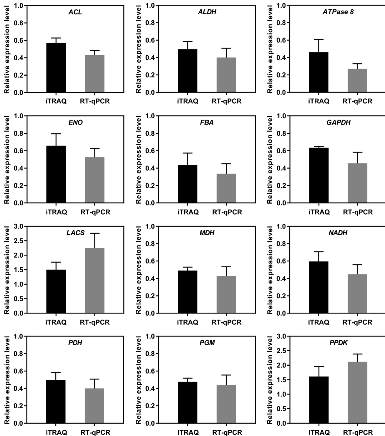
Fig. 8 Comparative analysis of mRNA and protein expression levels from RT-qPCR and iTRAQ analysis. The color bars represent the relative mRNA expression ratios of (MT/WT), values are means \pm SE ( n = 3 ) from the three replicates of RT-qPCR, asterisks above the bars indicate a significant difference at p < 0.05 .
