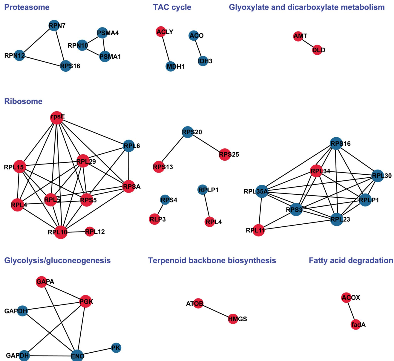
Fig. 7 Graphical representation of possible protein interaction network between MT and WT of S. miltiorrhiza . The node size represents the degree of proteins in the network. Node colors represent the upregulated and downregulated of the proteins with red and blue nodes, respectively. Edges (interactions) are the combination of any two nodes.
