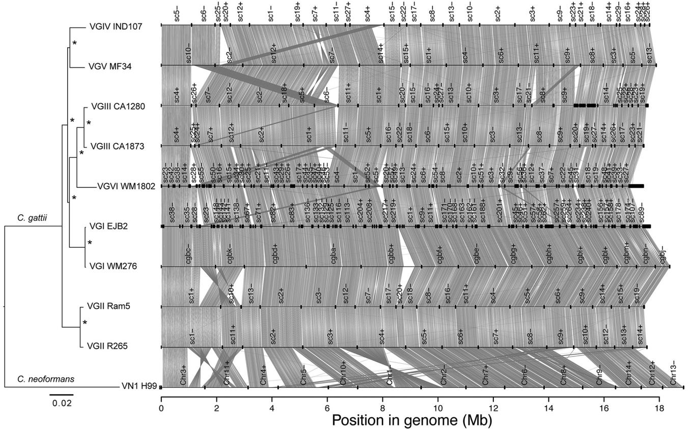
FIG 4 A phylogenetic tree for 10 Cryptococcus genomes belonging to the six C. gattii lineages and 1 C. neoformans lineage alongside their genome synteny. The phylogenetic tree was constructed in RAxML, with branch lengths indicating the mean number of nucleotide substitutions per site. To the right is a synteny plot, visualizing regions that span three or more orthologs between any two species as a connected gray line. Supercontig numbers are shown above each genome axis if longer than 400 kb, where a plus sign (+) represents the forward orientation and a minus sign (-) represents the negative orientation.
