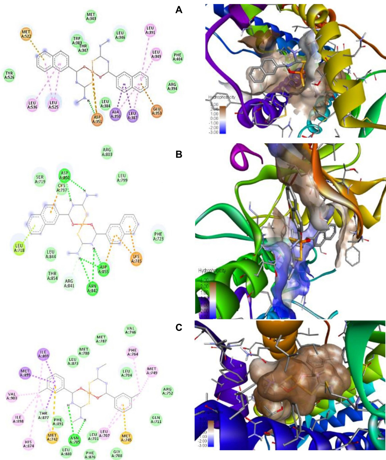
Figure 7 Visualisation of 2D (left) and 3D (right): Bis-(3-methyl-1-(naphthalene-2-carbonyl) thiourea) platinum (II)-3ERT complex ( A ); Bis-(3-methyl-1-(naphthalene-2-carbonyl) thiourea) platinum (II)-2I2O complex ( B ); Bis-(3-methyl-1-(naphthalene-2-carbonyl) thiourea) platinum (II)-1Z95 ( C ).
