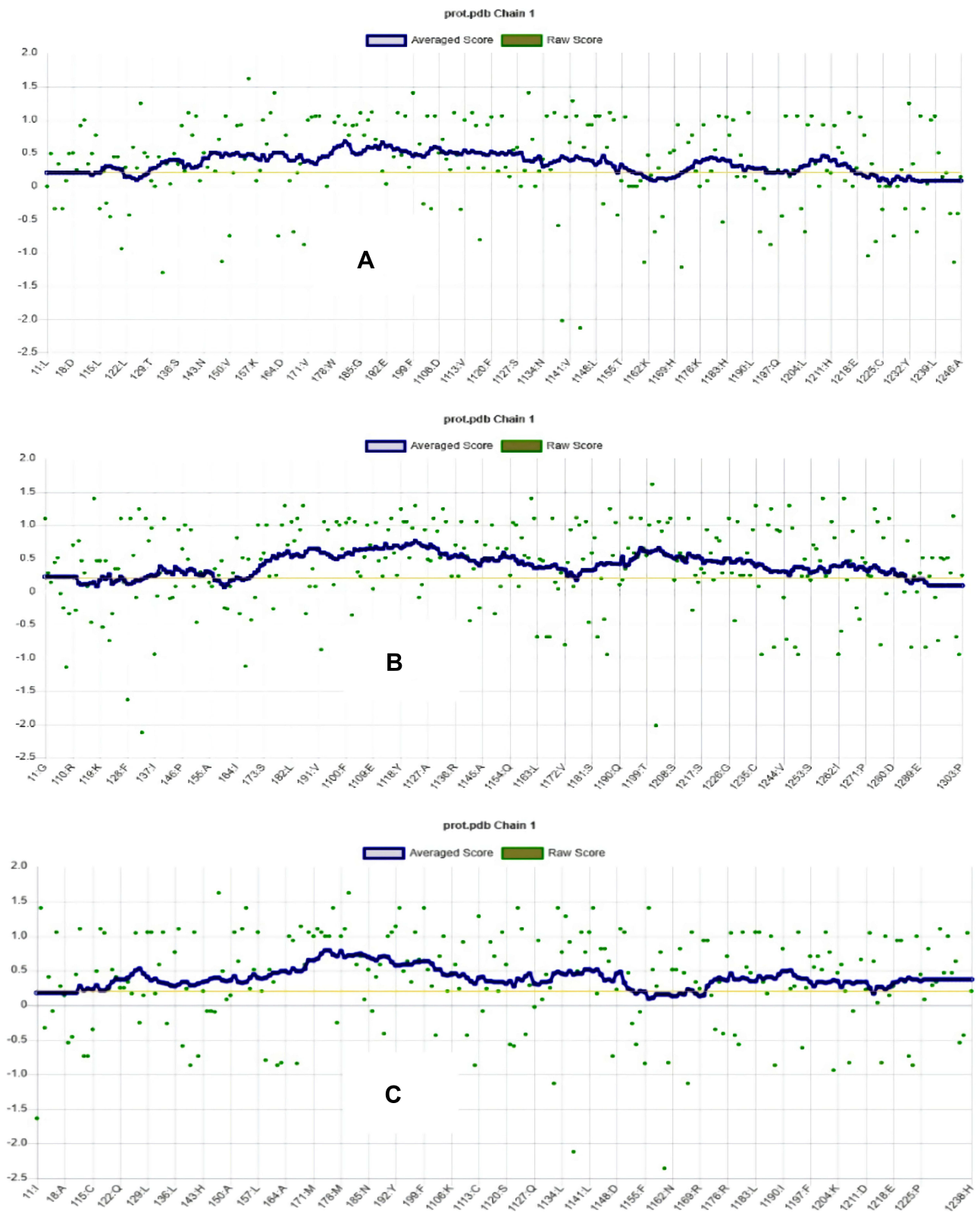
Figure 5 The 3D VERIFY analysis results of 3ERT (A); 2ITO (B); IZ95 (C).
