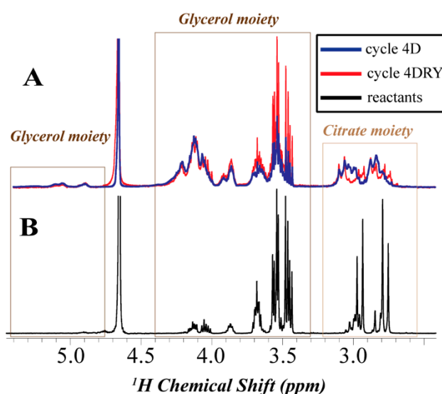
Figure 3. Representative ^1\text{H} NMR spectra of the glycerol-citric acid polymerization products in \text{D}_2\text{O} along with general peak assignments. (A) The overlaid spectra of the soluble fraction of the 4DRY sample [red] and the 4D sample [blue]; (B) The spectrum of the unreacted sample.
