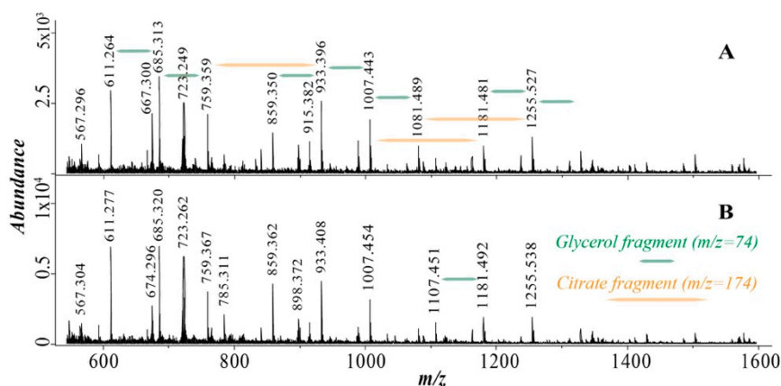
Figure 2. MALDI mass spectra of (A) the water-soluble fraction of the continuously dried sample collected after 8 periods (8DRY) and (B) cycled sample collected at the end of the experiment (8W). All labeled species correspond to (M + 23)^+ ions (sodium adducts).
