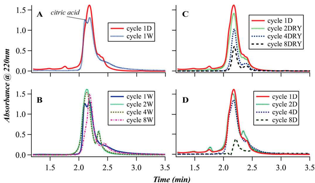
Figure 1. Size exclusion chromatography (SEC) analysis of the citric acid glycerol polymerization products (A) Comparison between the samples collected at the end of the first dry and wet cycle; (B) Comparison between the samples collected at the end of wet cycles (W series); (C) Comparison between samples of the DRY series; (D) Comparison of the samples collected at the end of dry period in the cycled series (D series).
