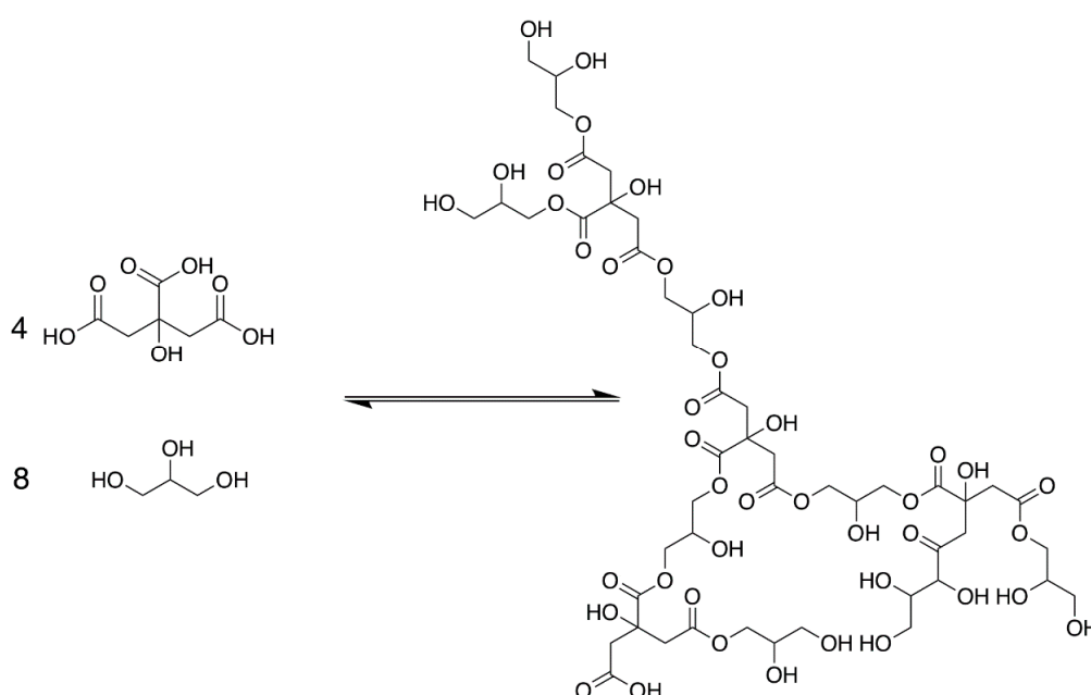
Scheme 1. Schematic representation of citric acid and glycerol polyesterification. The formation of one of the possible oligomers comprised from four citric acid and eight glycerol monomers is depicted. The polymerization is of A_3 + B_3 type. Here A refers to carboxylic acid groups, B refers to alcohol groups, subscript refers to the number of the functional group in each monomer.
