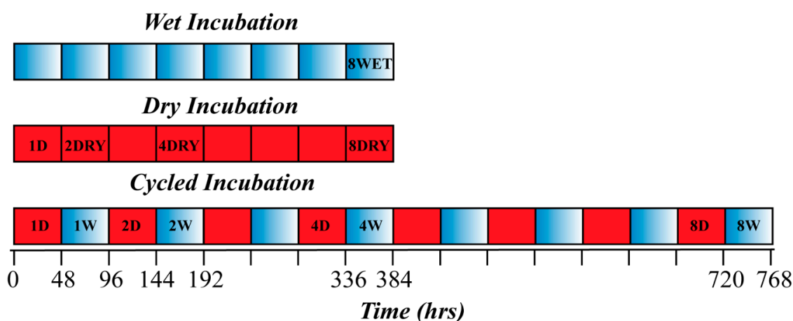
Scheme 2. Schematic representation of experimental setup and the sampling schedule. Red squares represents the dry heating period, blue-shaded squares represent the wet incubation period. The samples were collected at the end of labeled periods.
