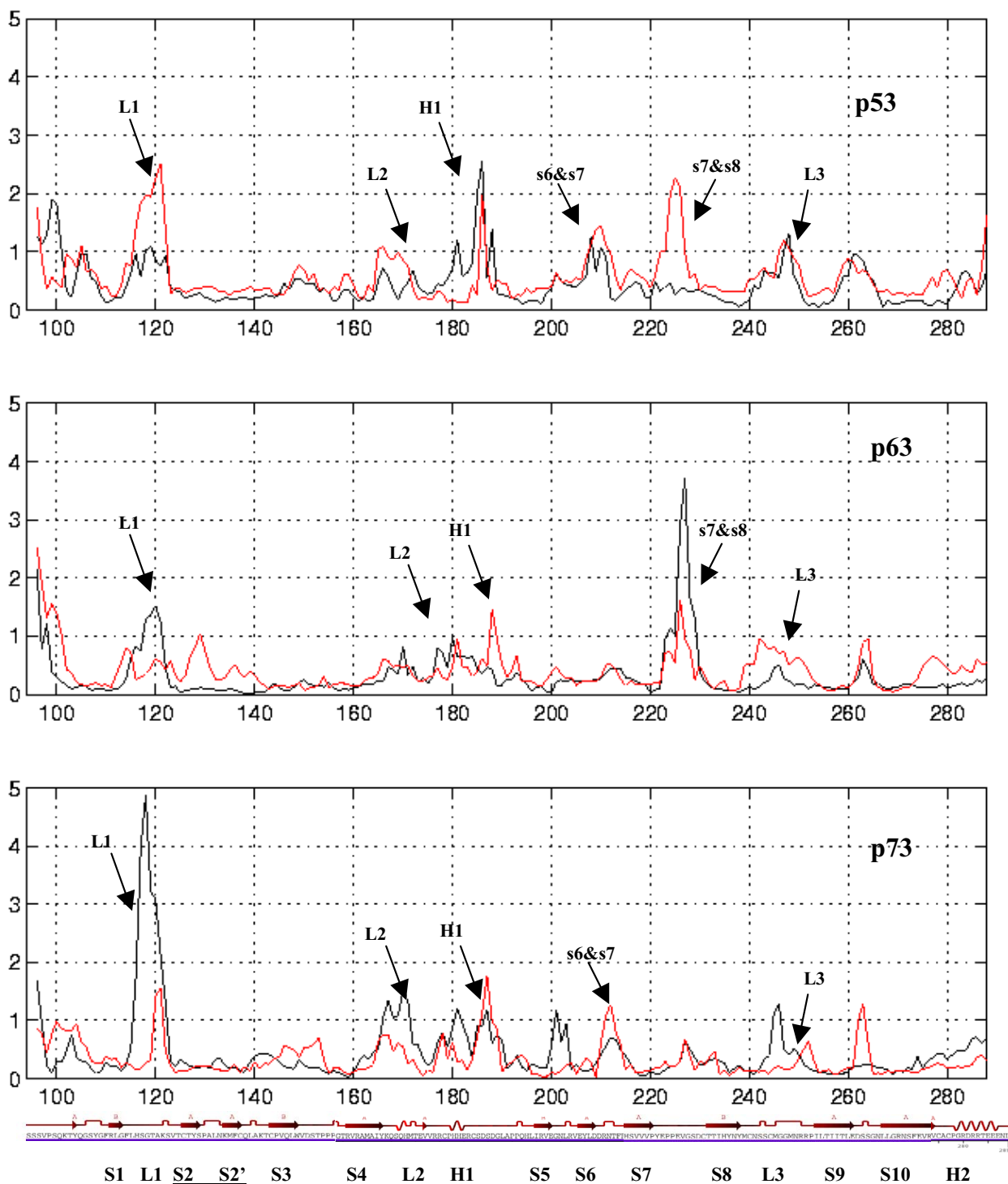
Figure 7 Projections on PCI. The RMSF of Cα atoms calculated after projecting the trajectories along their respective PCI directions (black – wild type; red – mutant).
