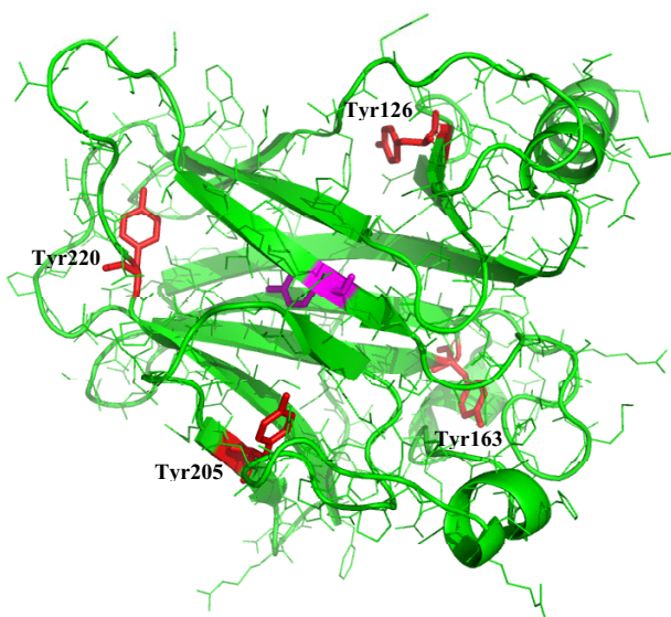
Figure 9 Structural plasticity. The structure of the core domain of p53 with the Tyr residues whose rates of flipping have been computed, shown as red sticks. Also shown is the core Tyr236 in magenta.
