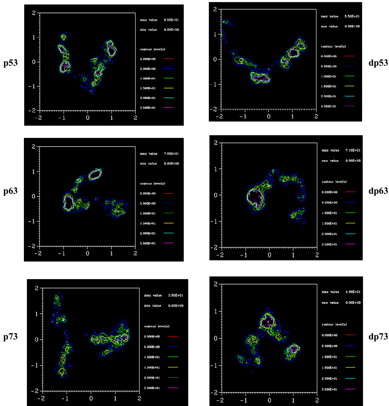
Figure 8 Conformational Sampling. The probability of sampling the phase space determined by principal modes 1 and 2 during the simulations of wild type (left) and mutant (right) p53, p63 and p73.
