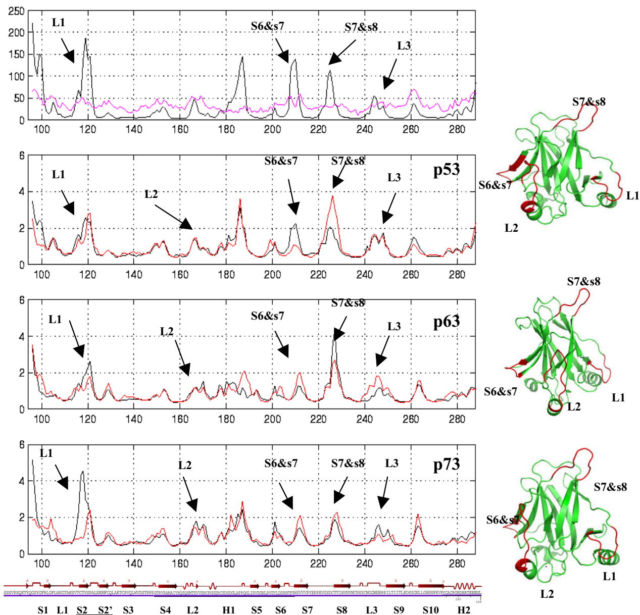
Figure 5 Fluctuations. Root mean squared fluctuations (RMSF) of the C- \alpha atoms during the simulations shown for the wild type (black) and mutant (red) p53, p63 and p73. In the top panel the experimental B-factors (magenta) are shown in comparison with the RMSF of the p53 simulations.
