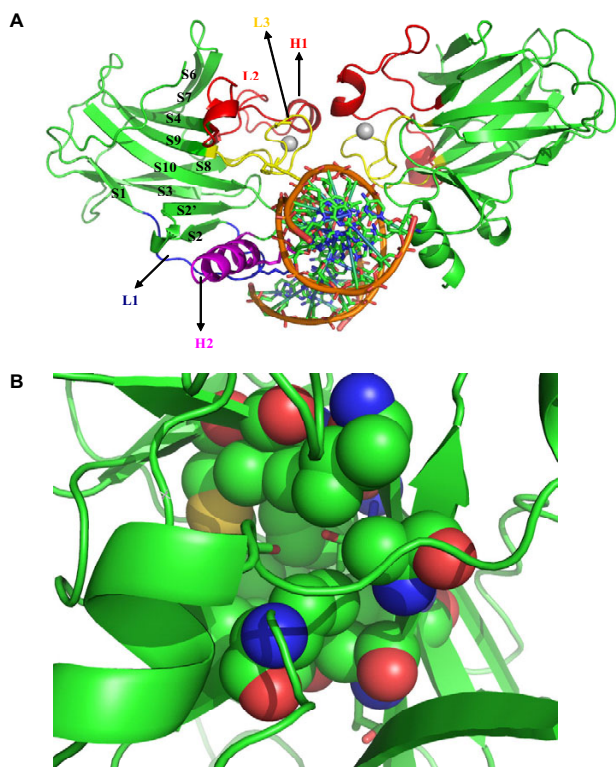
Figure 1 Structure of the Core domain. A. The structure of the p53 core domain in dimeric form complexed with DNA, taken from the crystal structure with RCSB code 2AHI [21]. Highlighted in magenta is the DNA binding helix H2, in red is the dimeric interface, blue is loop L1, yellow is loop L3. Zinc ion is represented as grey spheres; B. The two core residues Tyr236 and Thr253 shown in stick, surrounded in spheres by the predominantly hydrophobic core residues.
