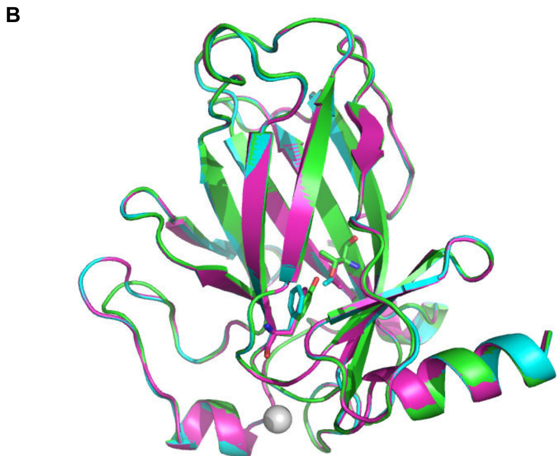
Figure 2 Sequence alignment. A. Multiple sequence alignment of the residues of the core domains of p53, p63, p73. Highlighted in red are the residues that have been mutated in this study and in blue are the Tyr residues whose mobilities have been examined. B. Superposition of the structures of the core domains of p53, p63 and p73 used in this study. Drawn in sticks are the residues that have been mutated in this study: Tyr236, Thr253.
