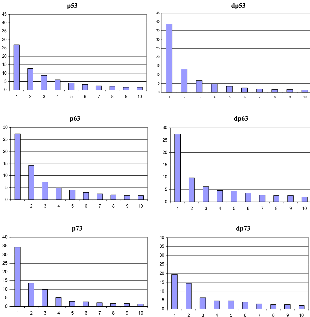
Figure 6 Principal Component Analysis. The percent contributions of the top 10 principal modes to the overall fluctuations during the simulations of wild type (left) and mutant (right) p53, p63 and p73.
