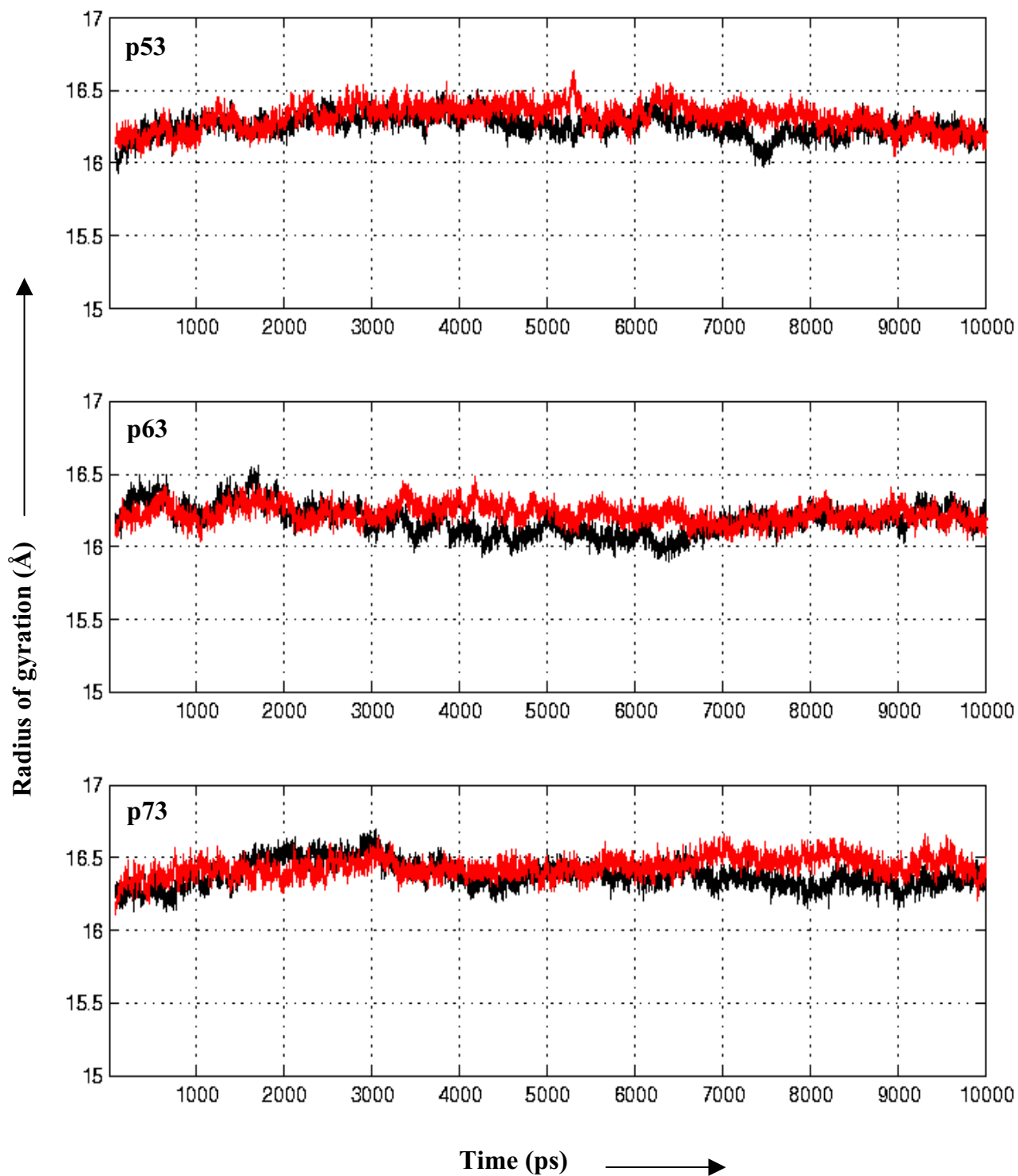
Figure 4 Radius of gyration. Radius of gyration as a function of time with respect to the starting structures during the MD simulations are shown for the wild type (black) and mutants (red) of p53, p63 and p73.
