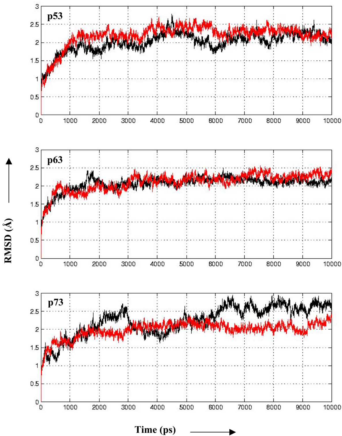
Figure 3 RMSD. Root Mean square Deviations (RMSD) of the backbone atoms as a function of time with respect to the starting structures during the MD simulations are shown for the wild type (black) and mutants (red) of p53, p63 and p73.
