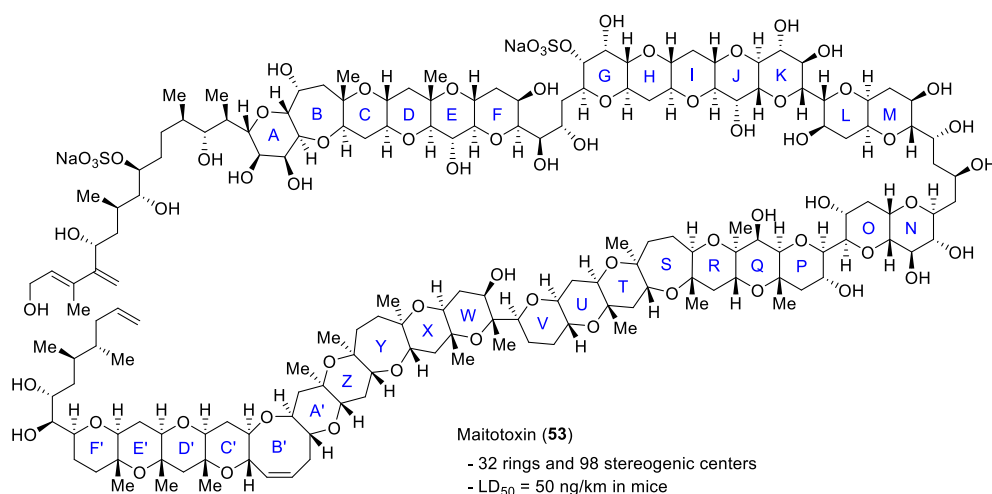
Figure 7. Structure of maitotoxin (53).
