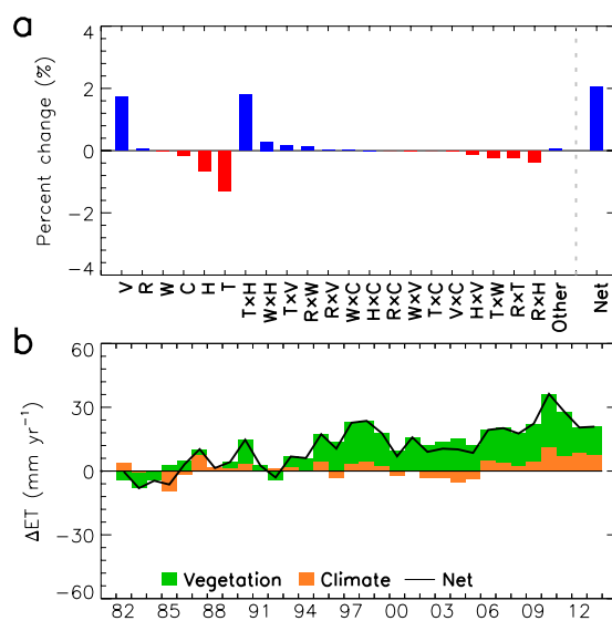
Figure 3. (a) Factorial contributions of vegetation dynamics (V), solar shortwave radiation (R), wind speed (W), atmospheric CO 2 concentration (C), actual air vapor pressure (H), air temperature (T), and their two-way and higher-order interactions affecting global land ET; (b) yearly contributions of the most influential factor, V, and sum of the other factors affecting global land ET. This figure was created using the IDL Core Version 7.1.2.
