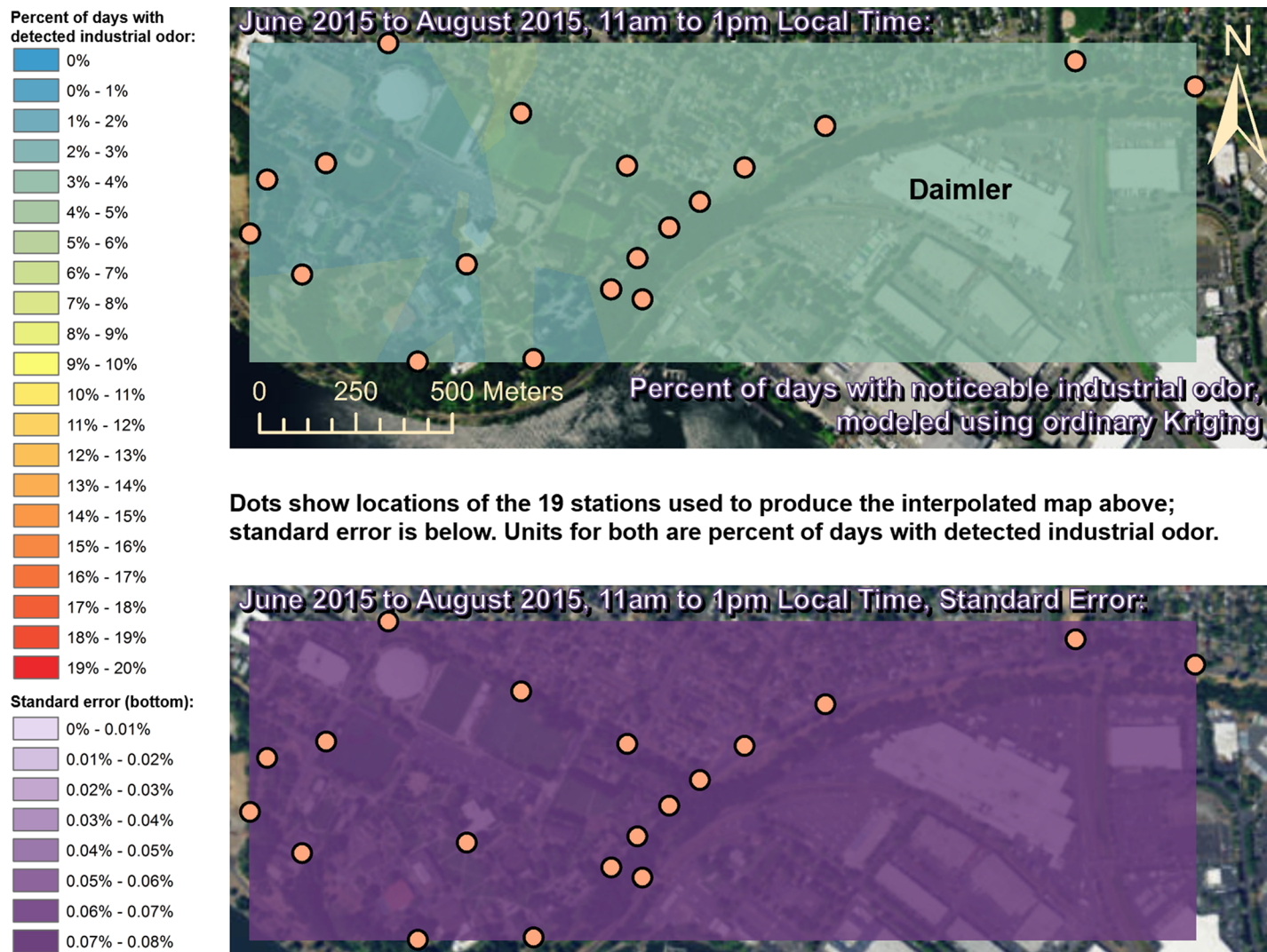
Fig 9. Frequencies of industrial odor detections (above) and standard error (below) during midday in summer. The spatial distribution of odor detections shows no clear pattern during this period. The bins here include all the values (no locations exceeded 20% of days with detected odors, or a standard error of 0.08%). Basemap from Esri's ArcGIS.
