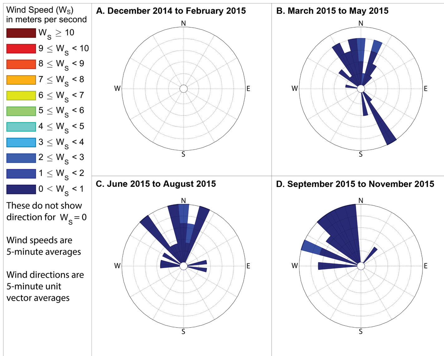
Fig 18. Winds measured between 11am and 1pm local time when food preparation odors were detected. These show directions from which the wind blew when food preparation odors were detected at either station 13 or 14 during midday in (A) winter, when no food preparation odors were detected, (B) spring, with the outermost ring representing a 10% frequency, (C) summer, with the outermost ring representing a 12% frequency, and (D) fall, with the outermost ring indicating a 12% frequency. These frequencies, and those stated in the text, include wind directions even when the measured wind speed was 0 \text{ m s}^{-1} , except where specifically indicated.
