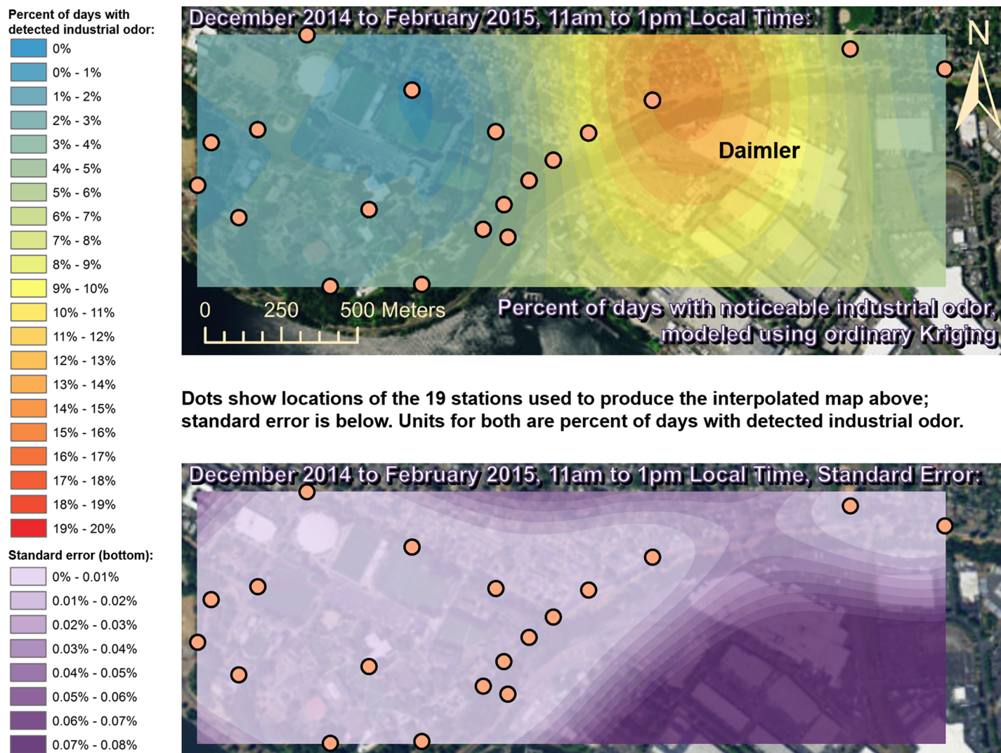
Fig 3. Frequencies of industrial odor detections (above) and standard error (below) during midday in winter. The areas northwest of the Daimler plant experienced far more industrial odors during this period than any other areas in the map according to both raw station data and the spatial interpolation here (above). These frequencies of odor detections are all much larger than the standard errors from the interpolation shown here (below) indicating a high signal-to-noise ratio. As expected, standard errors generally increase with increasing distance from the stations used to produce the interpolation (the dots shown here). The bins here include all the values (no locations exceeded 20% of days with detected odors, or a standard error of 0.08%). Basemap from Esri's ArcGIS.
