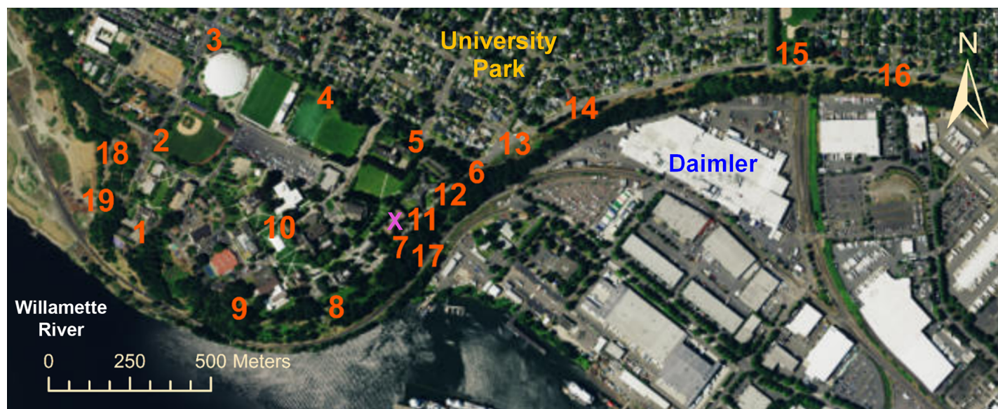
Fig 1. The study area in Portland, Oregon (USA). Orange numbers indicate locations of the 19 stations where this study collected odor data three times per day for one year. The blue label "Daimler" represents the location of the Daimler Trucks North America LLC plant this study hypothesized as producing industrial odors in the area. The yellow label "University Park" represents the location of a residential area on a bluff ~40 meters above the Daimler plant. The University of Portland campus is southwest of the University Park neighborhood. Odor detection stations were located subject to limited resources such as labor, and obstacles such as steep terrain and private property: all stations are either on public and easily accessible property, or on the University of Portland campus. The pink "X" shows the location of the automated weather station this study installed to measure wind speeds and directions in the area. Basemap from Esri's ArcGIS.
