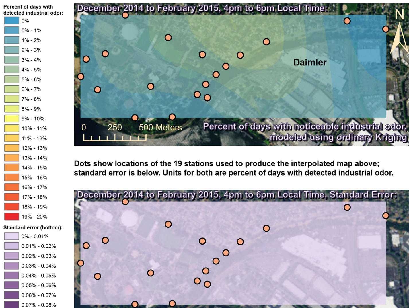
Fig 4. Frequencies of industrial odor detections (above) and standard error (below) during evening in winter. The areas northwest of the Daimler plant experienced slightly more industrial odors during this period than any other areas in the map according to both raw station data and the spatial interpolation here (above). These frequencies of odor detections are all much larger than the standard errors from the interpolation shown here (below) indicating a high signal-to-noise ratio. As expected, standard errors generally increase with increasing distance from the stations used to produce the interpolation (the dots shown here). The bins here include all the values (no locations exceeded 20% of days with detected odors, or a standard error of 0.08%). Basemap from Esri's ArcGIS.
