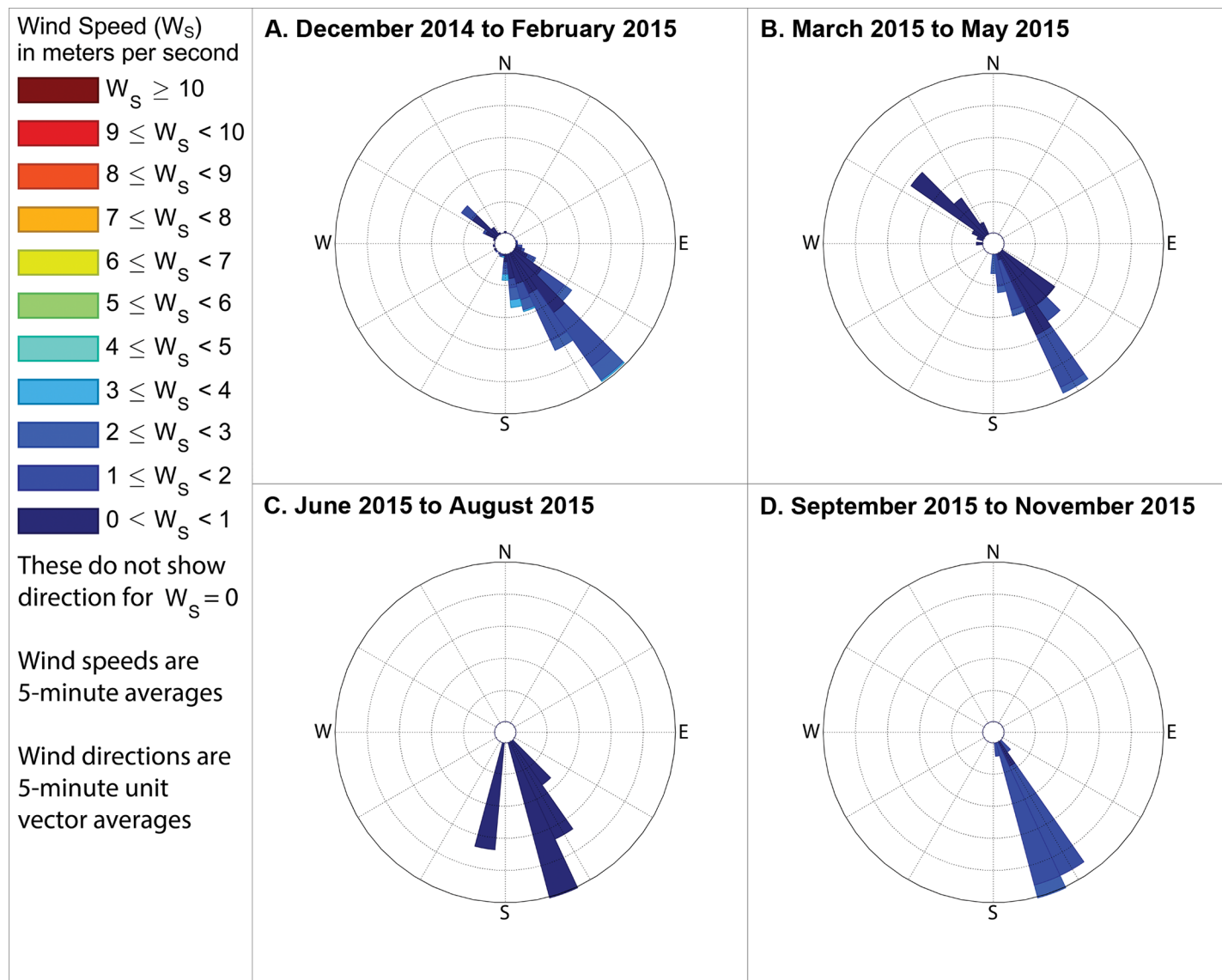
Fig 14. Winds measured between 6am and 8am local time when industrial odors were detected. These show directions from which the wind blew when industrial odors were detected at either station 13 or 14 during mornings in (A) winter, with the outermost ring indicating a 20% frequency, (B) spring, with the outermost ring representing a 10% frequency, (C) summer, with the outermost ring representing a 12% frequency, and (D) fall, with the outermost ring indicating a 24% frequency. These frequencies, and those stated in the text, include wind directions even when the measured wind speed was 0 \text{ m s}^{-1} , except where specifically indicated.
