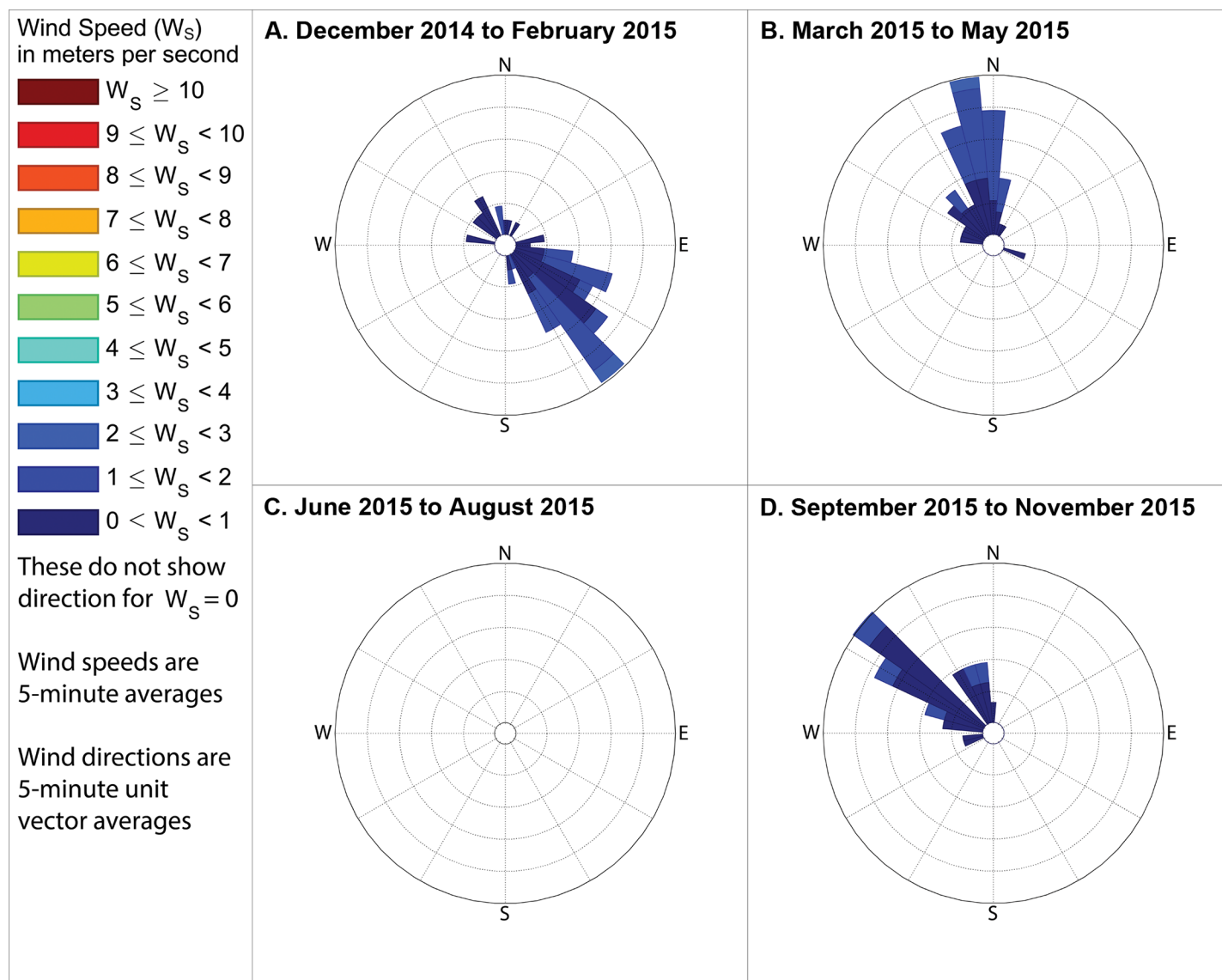
Fig 19. Winds measured between 4pm and 6pm local time when food preparation odors were detected. These show directions from which the wind blew when food preparation odors were detected at either station 13 or 14 during evenings in (A) winter, with the outermost ring indicating a 7% frequency, (B) spring, with the outermost ring representing a 19% frequency, (C) summer, when no food preparation odors were detected during the evening, and (D) fall, with the outermost ring indicating a 16% frequency. These frequencies, and those stated in the text, include wind directions even when the measured wind speed was 0 \text{ m s}^{-1} , except where specifically indicated.
