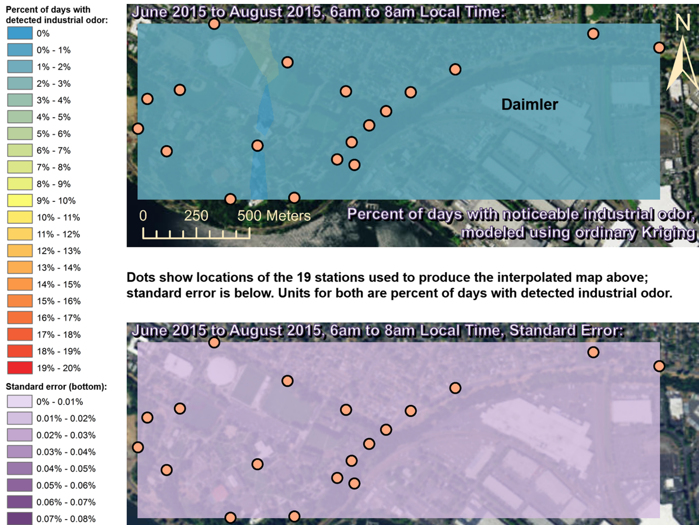
Fig 8. Frequencies of industrial odor detections (above) and standard error (below) during morning in summer. The spatial distribution of odor detections shows no clear pattern during this period. The bins here include all the values (no locations exceeded 20% of days with detected odors, or a standard error of 0.08%). Basemap from Esri's ArcGIS.
