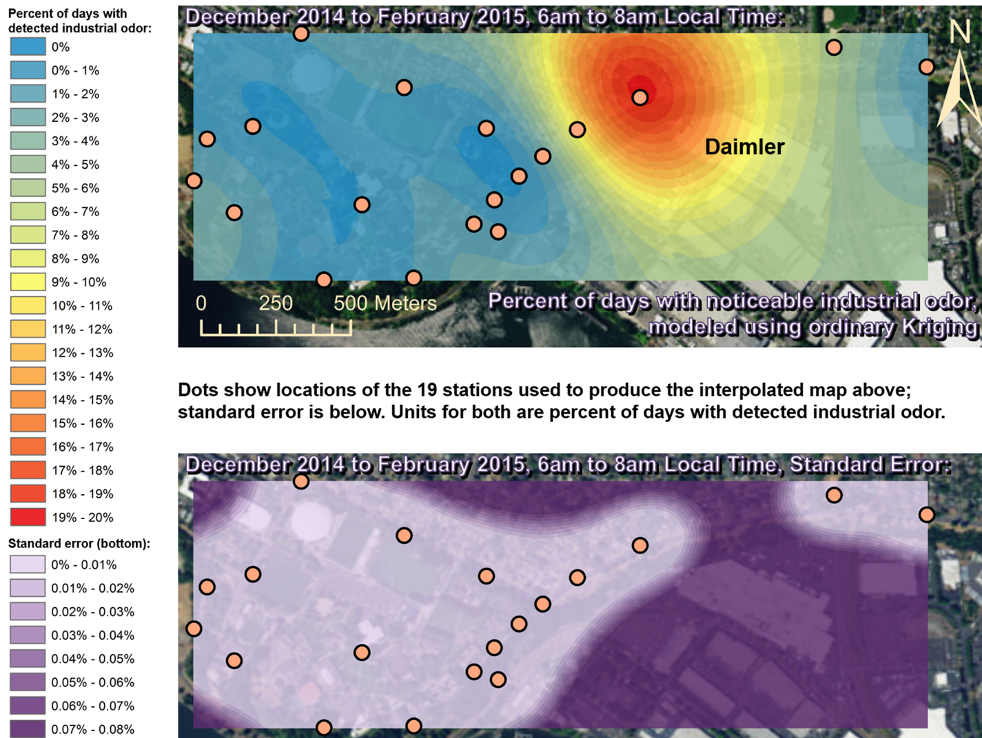
Fig 2. Frequencies of industrial odor detections (above) and standard error (below) during morning in winter. The areas northwest of the Daimler plant experienced far more industrial odors during this period than any other areas in the map according to both raw station data and the spatial interpolation here (above). These frequencies of odor detections are all much larger than the standard errors from the interpolation shown here (below) indicating a high signal-to-noise ratio. As expected, standard errors generally increase with increasing distance from the stations used to produce the interpolation (the dots shown here). The bins here include all the values (no locations exceeded 20% of days with detected odors, or a standard error of 0.08%). Basemap from Esri's ArcGIS.
