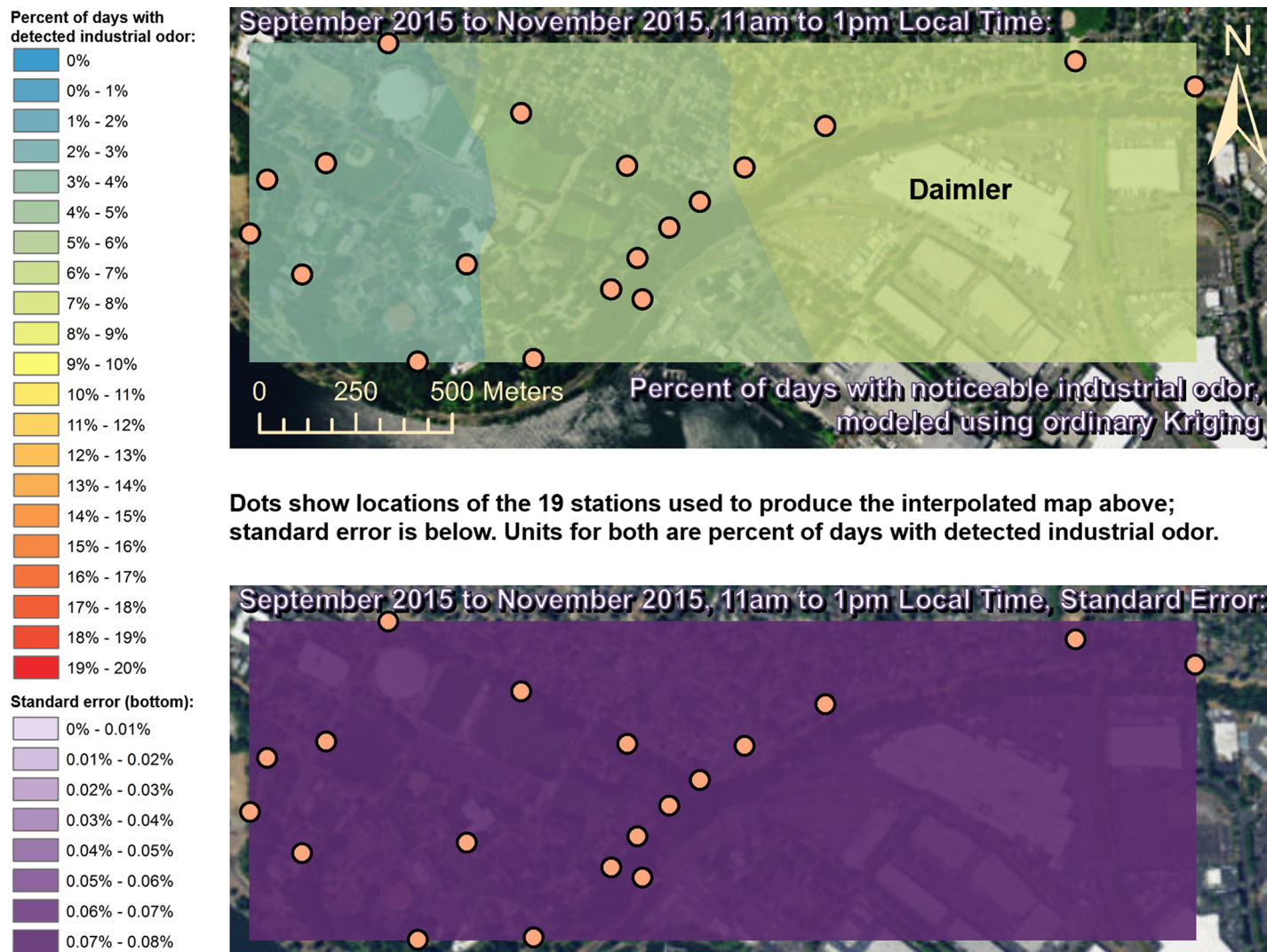
Fig 12. Frequencies of industrial odor detections (above) and standard error (below) during midday in fall. Odor detections generally decrease towards the western region of the map during this period. These frequencies of odor detections are all much larger than the standard errors from the interpolation shown here (below) indicating a high signal-to-noise ratio. As expected, standard errors generally increase with increasing distance from the stations used to produce the interpolation (the dots shown here). The bins here include all the values (no locations exceeded 20% of days with detected odors, or a standard error of 0.08%). Basemap from Esri's ArcGIS.
