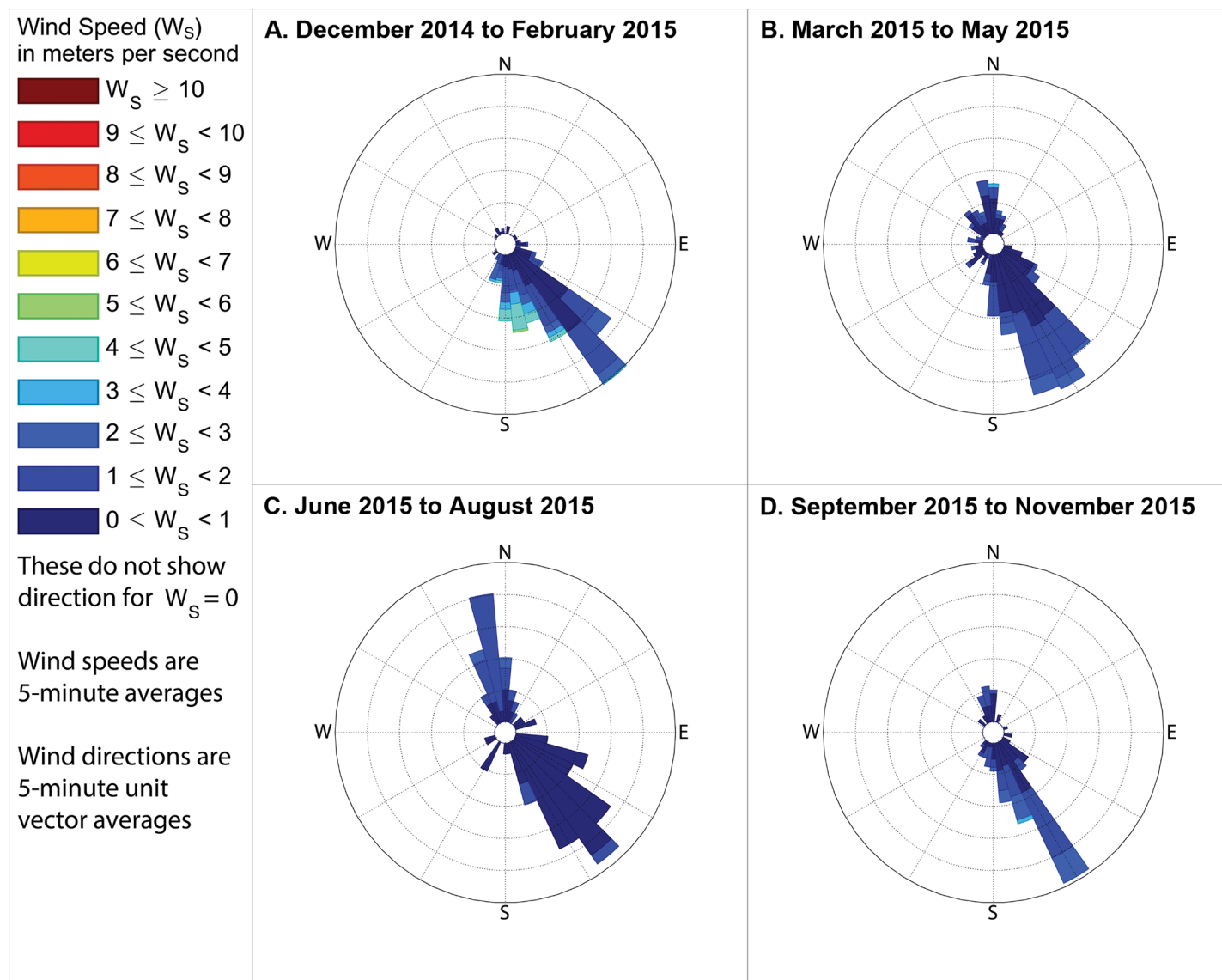
Fig 15. Winds measured between 11am and 1pm local time when industrial odors were detected. These show directions from which the wind blew when industrial odors were detected at either station 13 or 14 during midday in (A) winter, with the outermost ring indicating a 16% frequency, (B) spring, with the outermost ring representing an 11% frequency, (C) summer, with the outermost ring representing an 11% frequency, and (D) fall, with the outermost ring indicating a 20% frequency. These frequencies, and those stated in the text, include wind directions even when the measured wind speed was 0 \text{ m s}^{-1} , except where specifically indicated.
