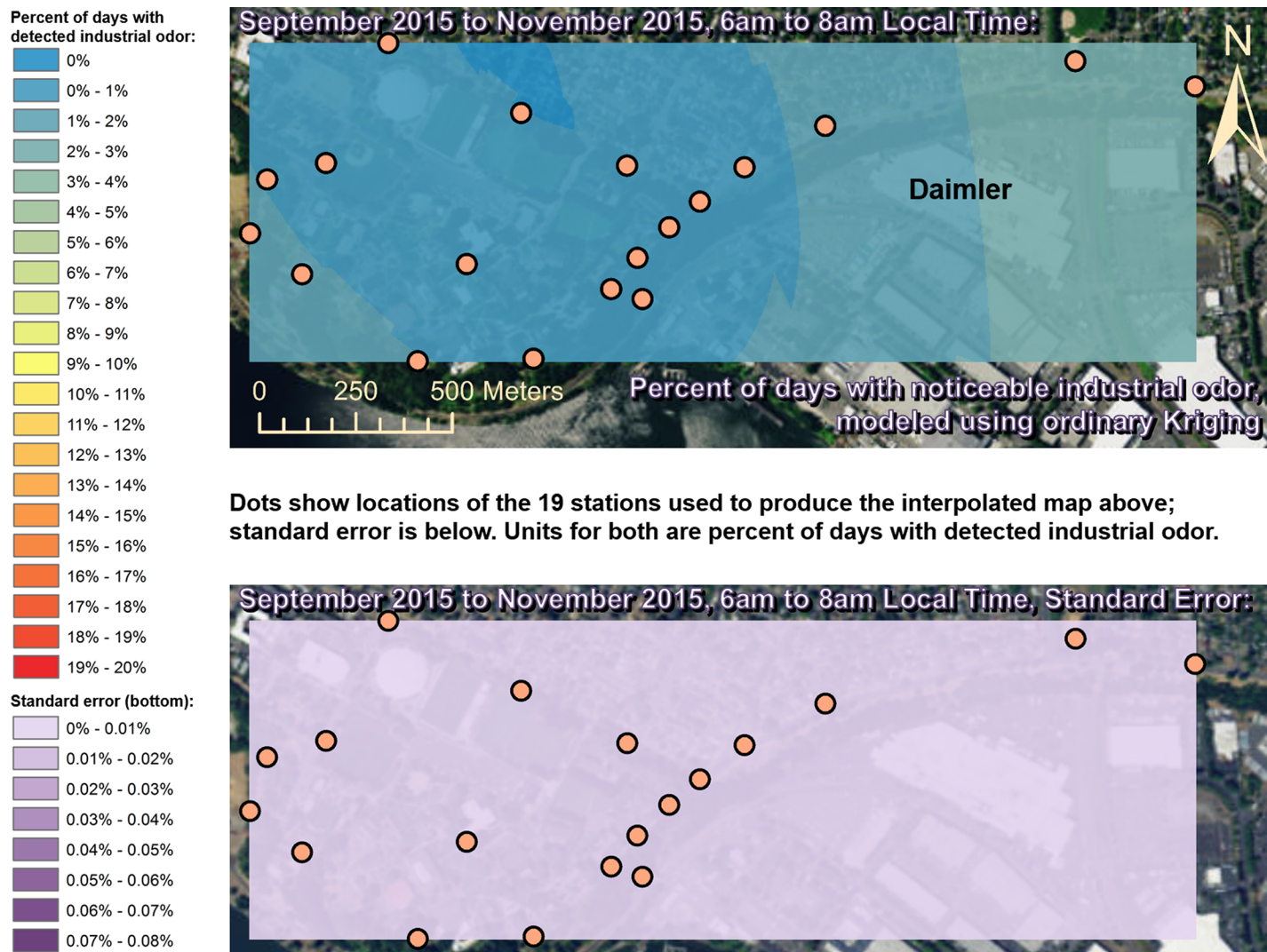
Fig 11. Frequencies of industrial odor detections (above) and standard error (below) during morning in fall. Odor detections generally decrease towards the northwest region of the map during this period. These frequencies of odor detections are all much larger than the standard errors from the interpolation shown here (below) indicating a high signal-to-noise ratio. As expected, standard errors generally increase with increasing distance from the stations used to produce the interpolation (the dots shown here). The bins here include all the values (no locations exceeded 20% of days with detected odors, or a standard error of 0.08%). Basemap from Esri's ArcGIS.
