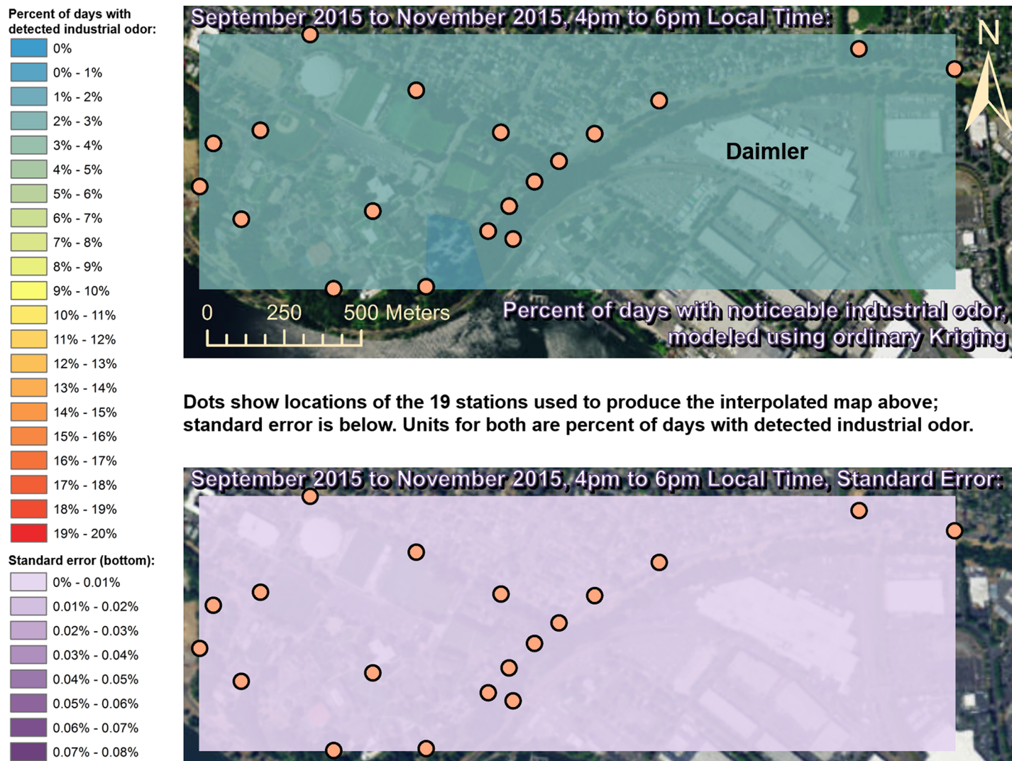
Fig 13. Frequencies of industrial odor detections (above) and standard error (below) during evening in fall. The spatial distribution of odor detections shows no clear pattern during this period. The bins here include all the values (no locations exceeded 20% of days with detected odors, or a standard error of 0.08%). Basemap from Esri's ArcGIS.
