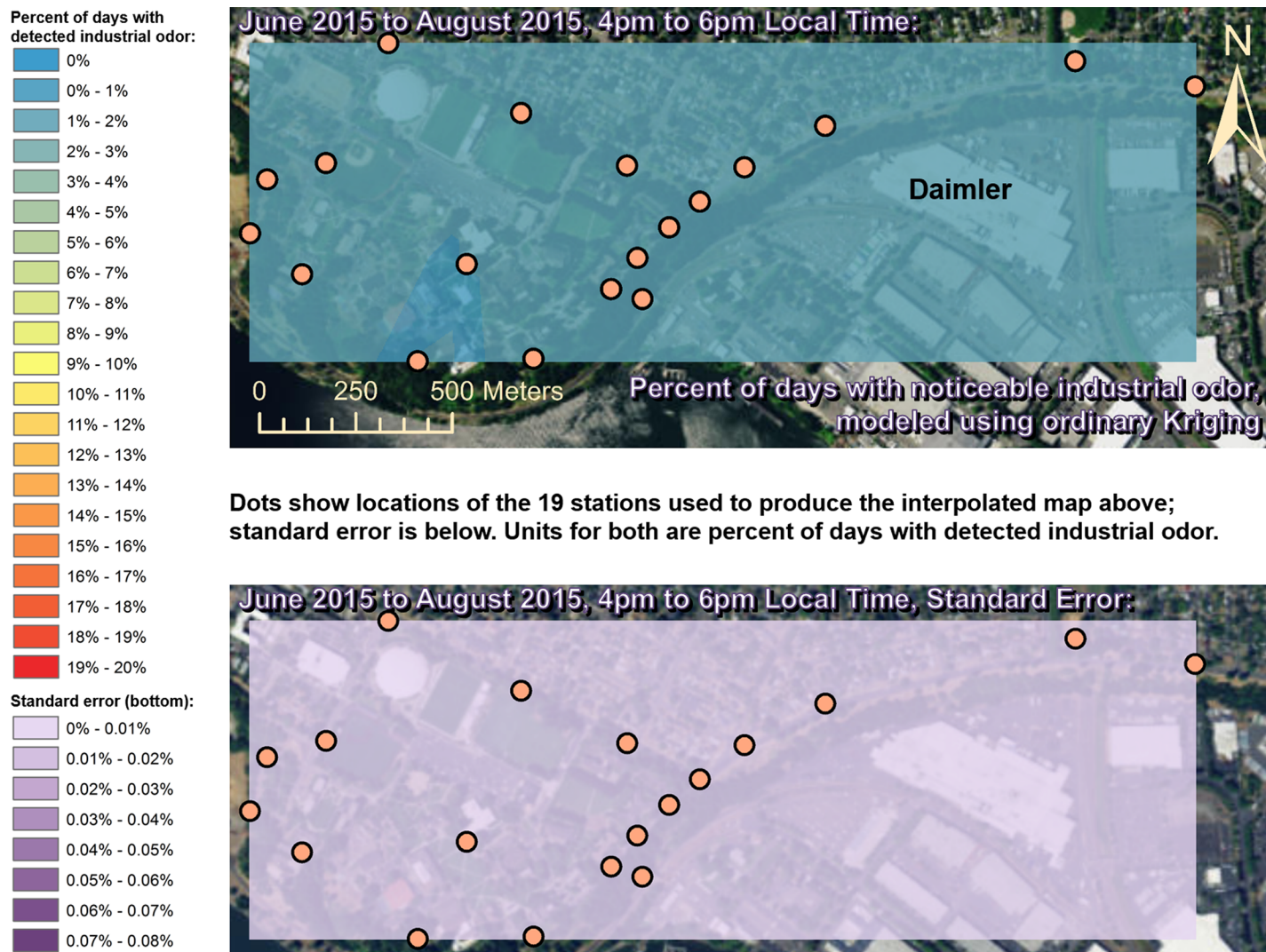
Fig 10. Frequencies of industrial odor detections (above) and standard error (below) during evening in summer. The spatial distribution of odor detections shows no clear pattern during this period. The bins here include all the values (no locations exceeded 20% of days with detected odors, or a standard error of 0.08%). Basemap from Esri's ArcGIS.
