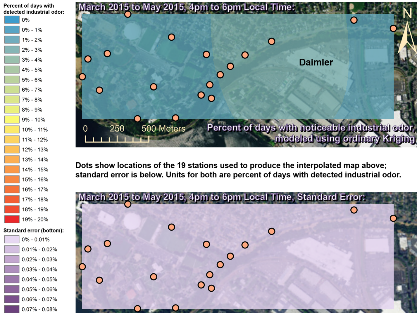
Fig 7. Frequencies of industrial odor detections (above) and standard error (below) during evening in spring. The areas surrounding the Daimler plant experienced slightly more industrial odors during this period than any other areas in the map according to both raw station data and the spatial interpolation here (above). These frequencies of odor detections are all much larger than the standard errors from the interpolation shown here (below) indicating a high signal-to-noise ratio. As expected, standard errors generally increase with increasing distance from the stations used to produce the interpolation (the dots shown here). The bins here include all the values (no locations exceeded 20% of days with detected odors, or a standard error of 0.08%). Basemap from Esri's ArcGIS.
