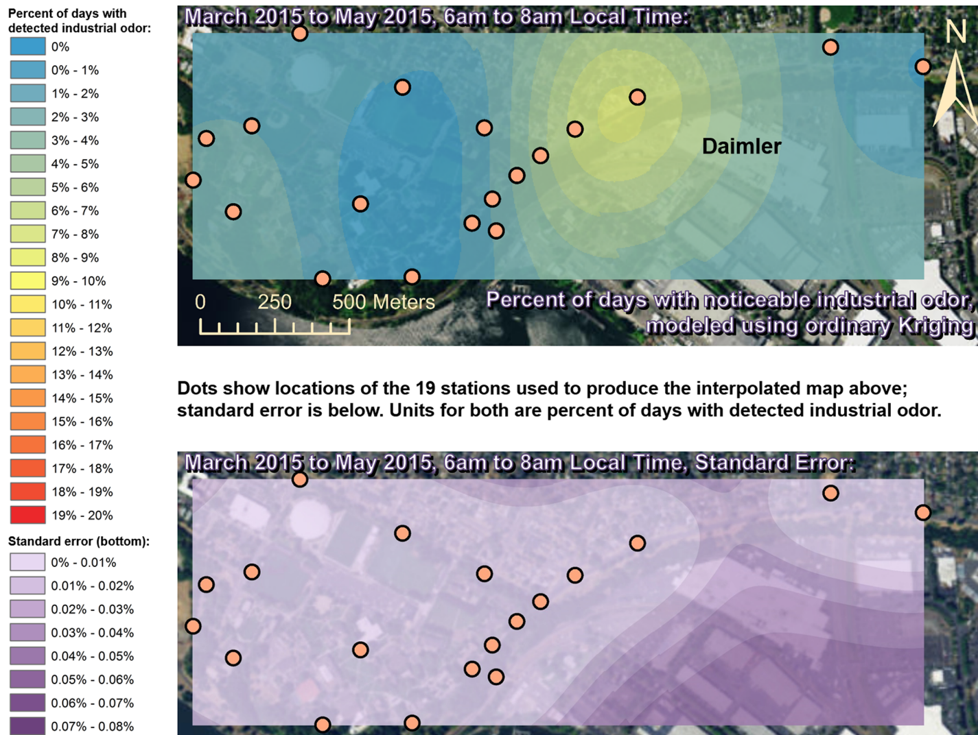
Fig 5. Frequencies of industrial odor detections (above) and standard error (below) during morning in spring. The areas northwest of the Daimler plant experienced far more industrial odors during this period than any other areas in the map according to both raw station data and the spatial interpolation here (above). These frequencies of odor detections are all much larger than the standard errors from the interpolation shown here (below) indicating a high signal-to-noise ratio. As expected, standard errors generally increase with increasing distance from the stations used to produce the interpolation (the dots shown here). The bins here include all the values (no locations exceeded 20% of days with detected odors, or a standard error of 0.08%). Basemap from Esri's ArcGIS.
