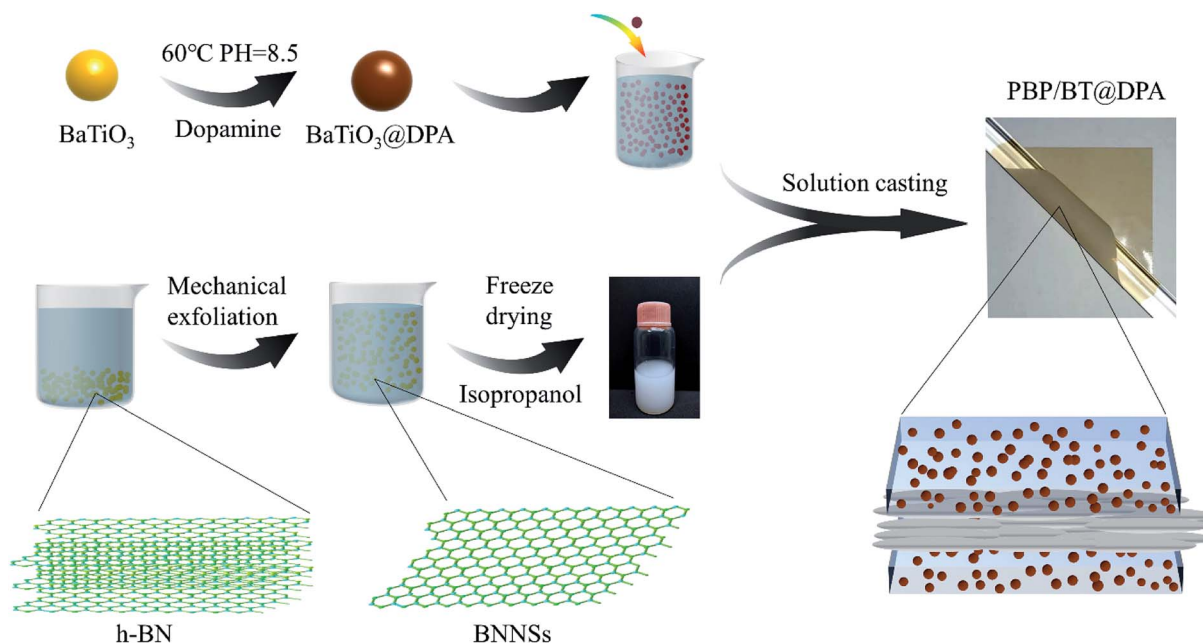
Fig. 1 Experimental flow chart: surface modification of \text{BaTiO}_3 by dopamine, preparation of BNNSs and fabrication of sandwich structure film.
