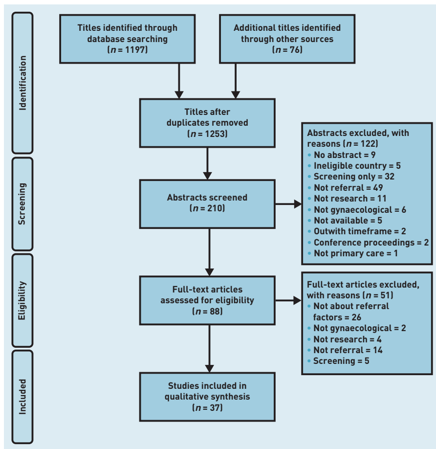
Figure 2. PRISMA diagram.
