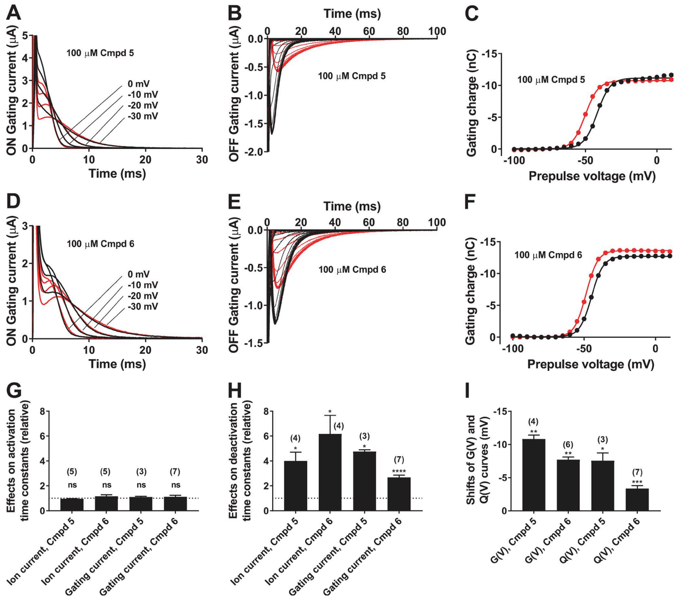
Figure 5. Effects on the gating currents of the W434F Shaker K_v channel. (A) Effect of 100 \mu M Cmpd 5 on the ON-gating currents at denoted voltages. Holding voltage, -80 mV; extracellular solution, 1K; black curves, control solution; red curves, compound solution. (B) Effect of 100 \mu M Cmpd 5 on the OFF-gating currents at -80 mV, after 500-ms prepulses between -100 and +10 mV in steps of 5 mV. Extracellular solution, 1K; black curves, control solution; red curves, compound solution. (C) Effect of 100 \mu M Cmpd 5 on gating charge versus voltage, Q(V) , curve. Extracellular solution, 1K. The gating charges were calculated as the area under the curve in B from 1.5 to 100 ms. Black symbols and curves, control solution; red symbols and curves, compound solution. Data were fitted to Eq. 2 (with exponent n = 1 ). \Delta V_{1/2} = -8.3 mV. (D) Same as in A but Cmpd 6. (E) Same as in B but Cmpd 6. (F) Same as in C but Cmpd 6. \Delta V_{1/2} = -3.8 mV. (G–I) Effects of 100 \mu M Cmpd 5 and 6 on the activation time constant (G), the deactivation time constant (H), and the steady-state curves (I). Channel activation is measured as the opening in Fig. 4 (A and D) and as the single exponential relaxation phase (as recorded in Fig. 5 A at 0 mV). Channel closing is measured as the closing in Fig. 4 (B and E) and as the single exponential relaxation phase at -80 mV after a prepulse to 0 mV as recorded in Fig. 5 (B and E). Shifts of G(V) (from Fig. 2 C), and Q(V) as measured in Fig. 5 (C and F). Mean \pm SEM. Number of experiments indicated in the figure. A two-tailed t test was used to compare effects to a hypothetical value of 1 in G and H and 0 in I. ns, P > 0.05 ; *, P < 0.05 ; **, P < 0.01 ; ***, P < 0.001 ; ****, P < 0.0001 .
