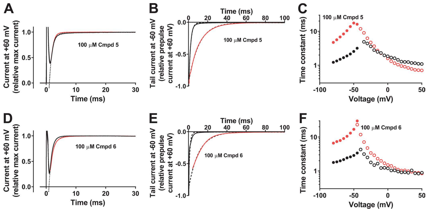
Figure 4. Effects on the opening and closing kinetics of the WT Shaker K_V channel. (A) Effect of 100 \mu\text{M} Cmpd 5 on the opening at +60 mV. Holding voltage, -80 mV; extracellular solution, 100K; black curve, control solution; red curve, compound solution. Single exponential curves (dashed lines) were fitted from 1.5 to 30 ms. \tau(\text{control}) = 1.01 ms, \tau(\text{Cmpd 5}) = 0.88 ms. (B) Effect of 100 \mu\text{M} Cmpd 5 on the closing at -60 mV. Prepulse voltage = +60 mV for 100 ms. Extracellular solution, 100K; black curve, control solution; red curve, compound solution. Tail currents were normalized to the current at the end of the activation pulse. Single exponential curves (dashed lines) were fitted to the tail currents after removal of capacitive spikes. \tau(\text{control}) = 1.88 ms, \tau(\text{Cmpd 5}) = 10.8 ms. (C) Effect of 100 \mu\text{M} Cmpd 5 on time constants at different voltages. Time constants for channel opening (as in A but 1K solution, open symbols). Time constants for channel closing (as in B, closed symbols). Black symbols, control solution; red symbols, compound solution. (D) Same as in A but Cmpd 6. \tau(\text{control}) = 0.89 ms, \tau(\text{Cmpd 6}) = 1.20 ms. (E) Same as in B but Cmpd 6. \tau(\text{control}) = 1.22 ms, \tau(\text{Cmpd 6}) = 10.6 ms. (F) Same as in C but Cmpd 6.
