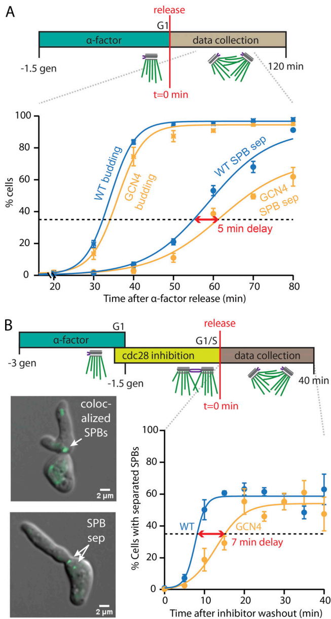
Figure 4. Microtubule pivoting flexibility specifically affects rate of pole separation. (A) Timing of bud emergence and SPB separation for cdc28-as1 cells expressing GCN4 (gold) versus WT (blue) Spc110 after release from G1 using \alpha -factor alone. Cells were synchronized in G1 with single, unduplicated SPBs using \alpha -factor for 1.5 generation (gen)-times. For each time point after release, percentages of cells with buds or with separated SPBs were counted. SPB separation (sep) was delayed in GCN4 cells by 5 min relative to WT cells. (B) Timing of bud emergence and SPB separation for cdc28-as1 cells expressing GCN4 (gold) versus WT (blue) Spc110 after release from G1/S using the double-synchronization protocol. Cells were initially synchronized with single SPBs using \alpha -factor alone and then transferred into 1NM-PP1 alone to allow SPB duplication and insertion. For each time point after release, percentages of cells with separated SPBs were counted. SPB separation was delayed in GCN4 cells by 7 min relative to WT cells. Inset: Representative images of cdc28-as1 cells expressing WT Spc110. Immediately after release from G1/S, the duplicated SPBs are colocalized at the bud neck ( t = 0 min, top) and appear as a single green spot. Later ( t = 20 min, bottom), the SPBs are separated (sep). Hyperpolarized cell shape is characteristic of Cdc28-as1 inhibition (Bishop et al., 2000; Crasta et al., 2006). Symbols and error bars in A and B represent mean \pm SD (from n = 3 cultures). Horizontal dotted lines indicate 35% thresholds used to compare SPB separation timing across strains.
