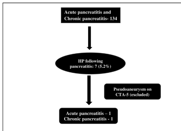
Fig. 2 Inclusion flowchart.
