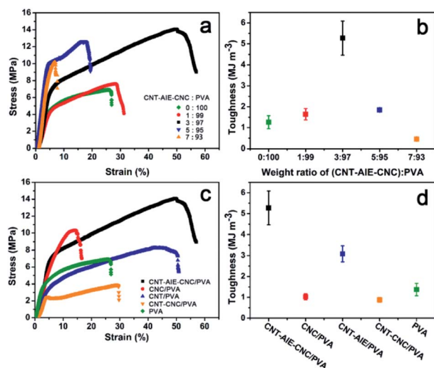
Fig. 3 Characterizing the mechanical properties of CNT-AIE-CNC/PVA with varying weight ratio of (CNT-AIE-CNC) : PVA: (a) stress-strain curves. (b) Toughness. (c) Comparing the mechanical properties of CNT-AIE-CNC/PVA with other filler : PVA electrospun fibers (CNC/PVA, CNT-AIE/PVA, CNT-CNC/PVA, PVA): (c) stress-strain curves. (d) Toughness.
